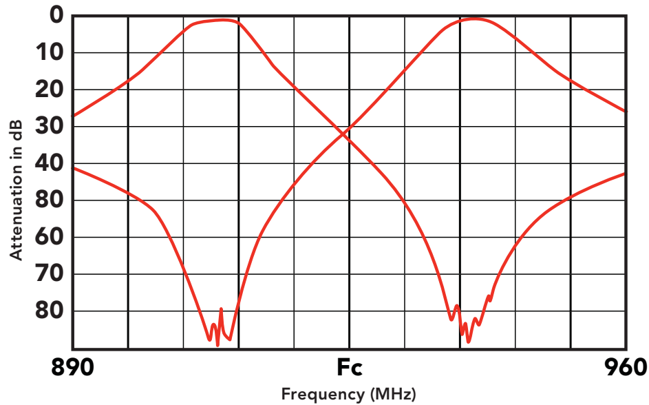
TYPICAL RESPONSE
