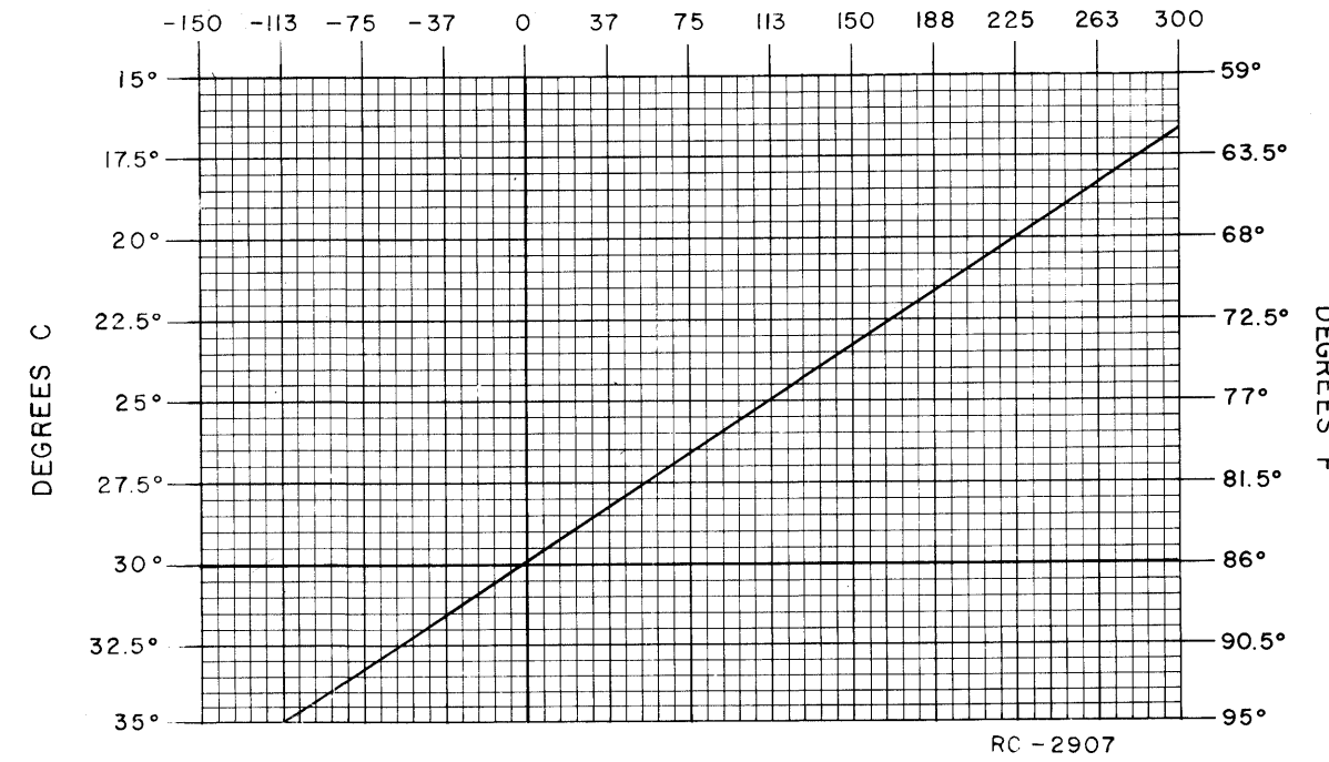
Figure 4 - Frequency Characteristics Vs. Temperature
