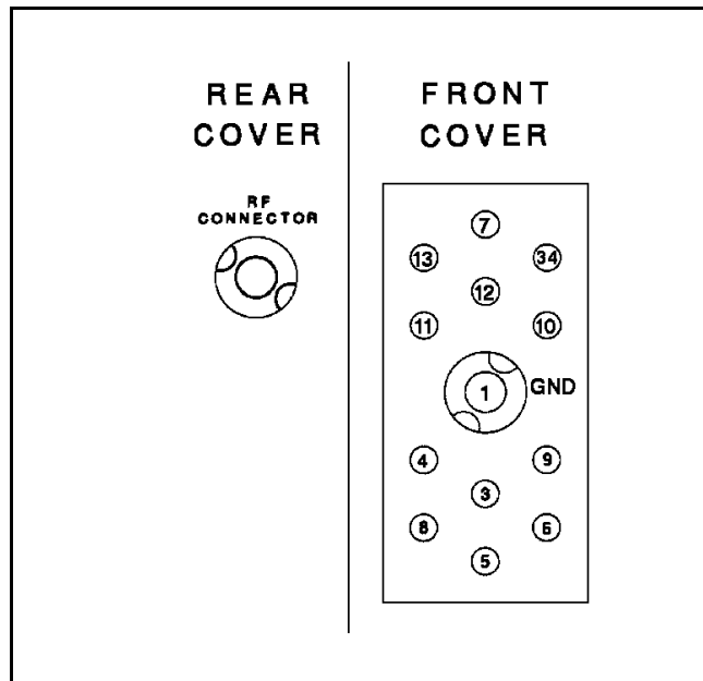
Figure 6 - UDC Pin-Out
