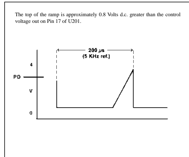
Figure 5 - Ramp (Generated In U201 And Appears On Pin 15)
