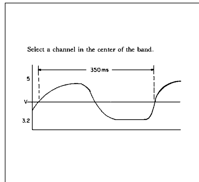
Figure 4 - F_{in} (Input To U201, Pin 10)
