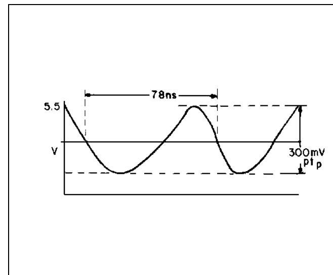
Figure 3 - Reference Oscillator (Input To PLL Module U201, Pin 2)
