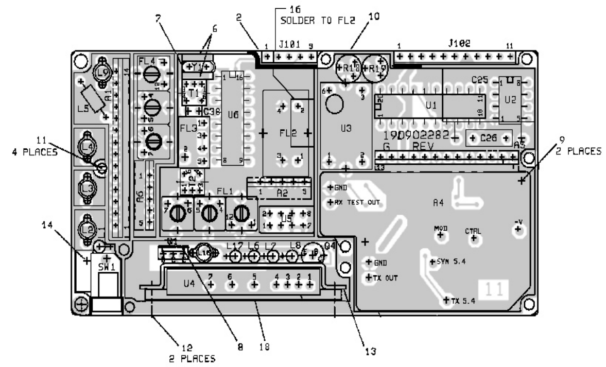
(19D902282, Sh. 2, Rev. 11) (19D902283, Comp. Side, Rev. 11)
