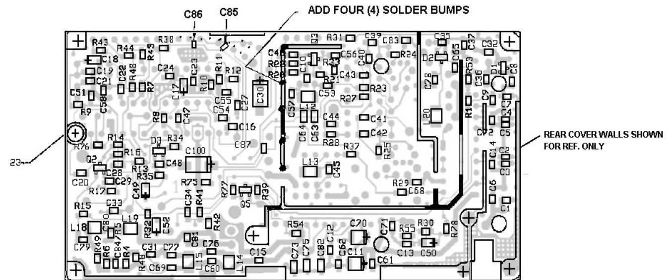
(19D902282, Sh. 2, Rev. 15) (19D902283, Solder Side, Rev. 11)
