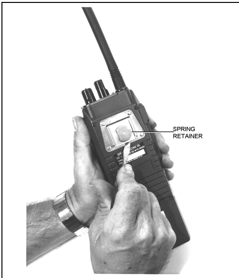
Figure 10 - Swivel Mount Removal And Replacement
