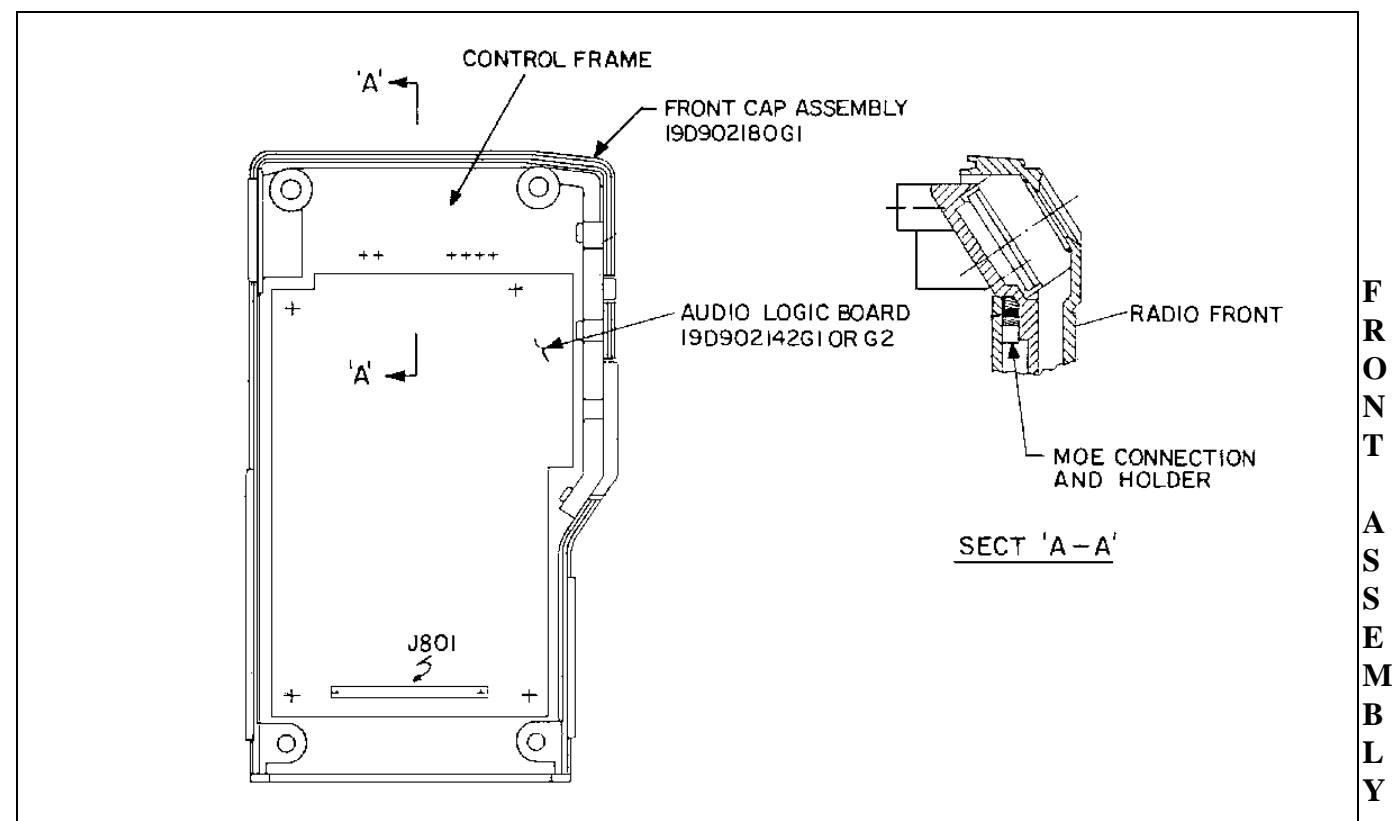
Figure 1 - Radio Front Assembly
