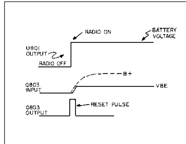
Figure 5 - Voltage Waveforms
