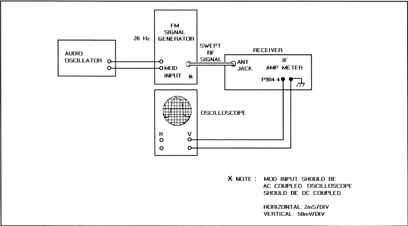
Figure 6 - Test Setup for 20 Hz Double-Trace Sweep Alignment
