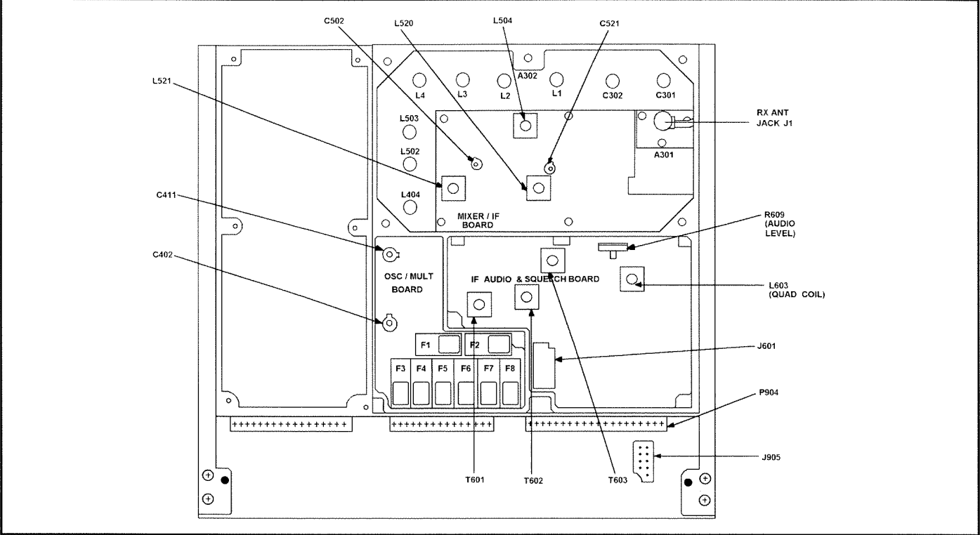
Figure 5 - Test Points And Alignment Controls
