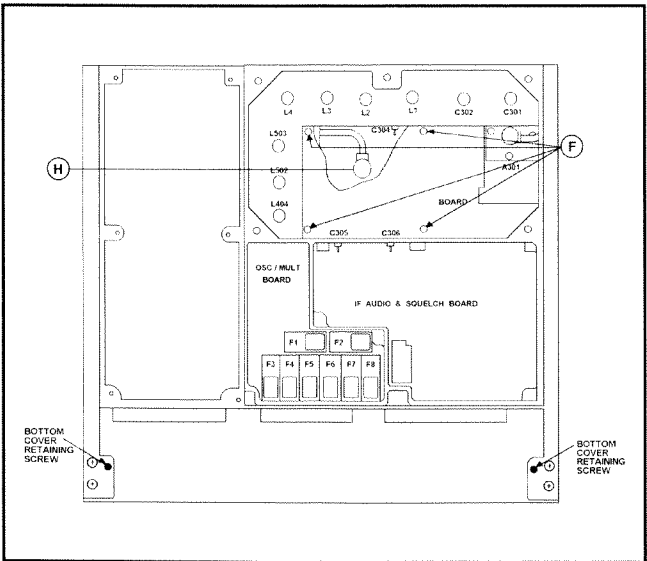
Figure 1 - Disassembly Procedure (Top View)
