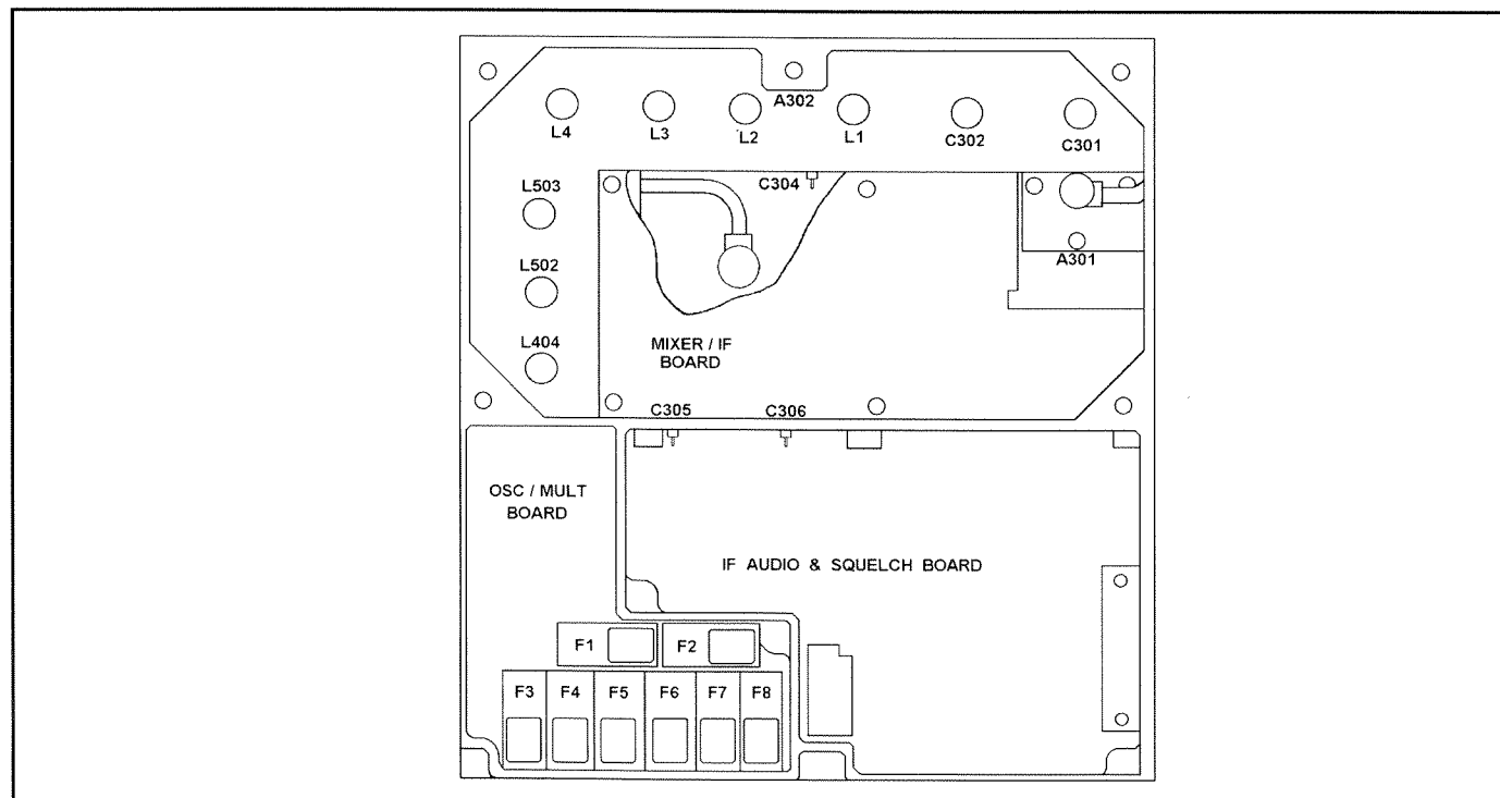
Figure 4 - Receiver Module Location Diagram
