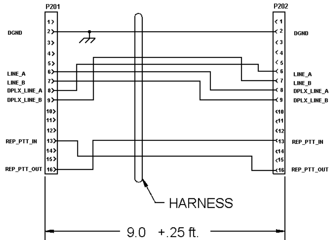
MASTR III BACK TO BACK REPEATER HARNESS
