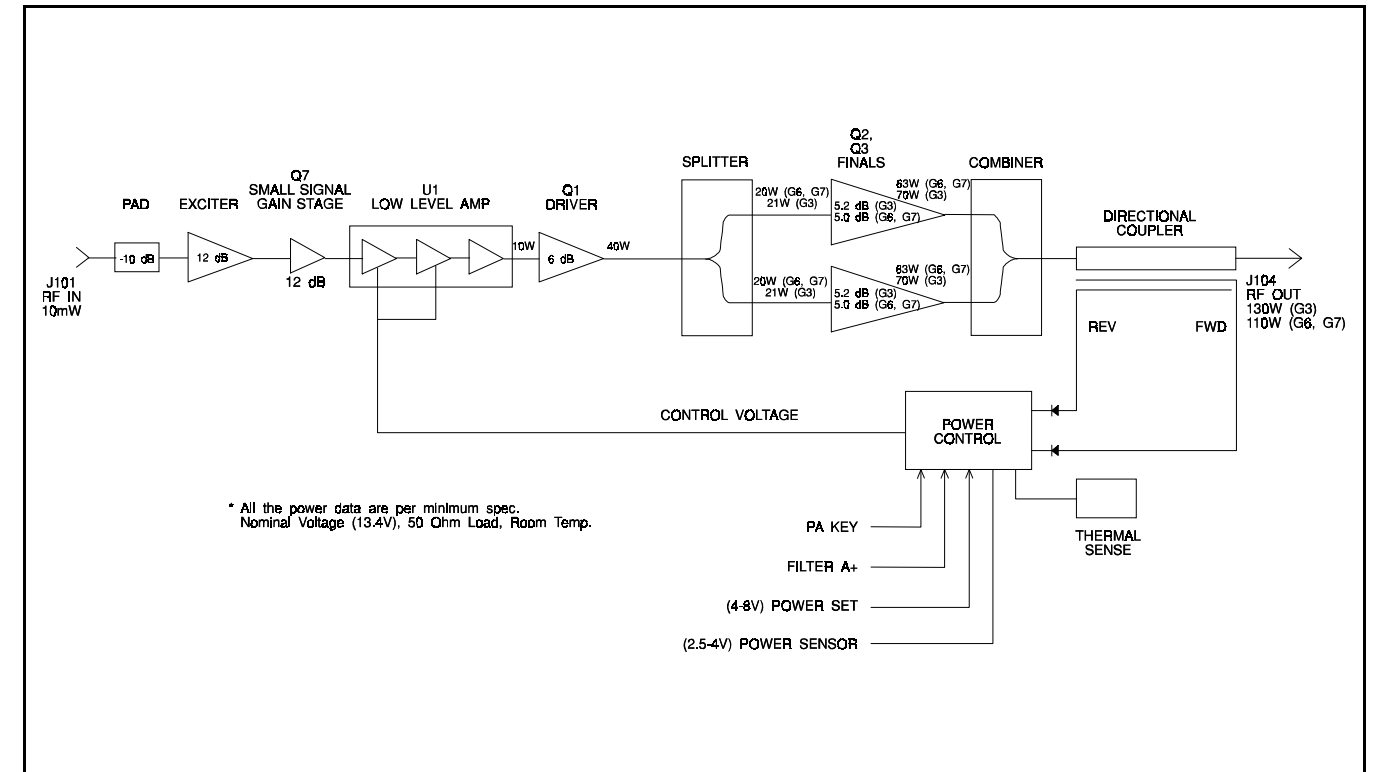
Figure 1 - Block Diagram
