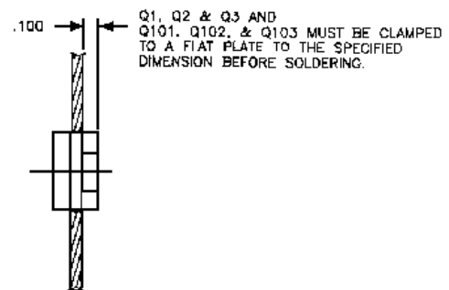
VIEW G TYPICAL LEAD FORMING & ASSEMBLY POSITIONING FOR Q1 THRU Q3 FOR Q101 THRU Q103
