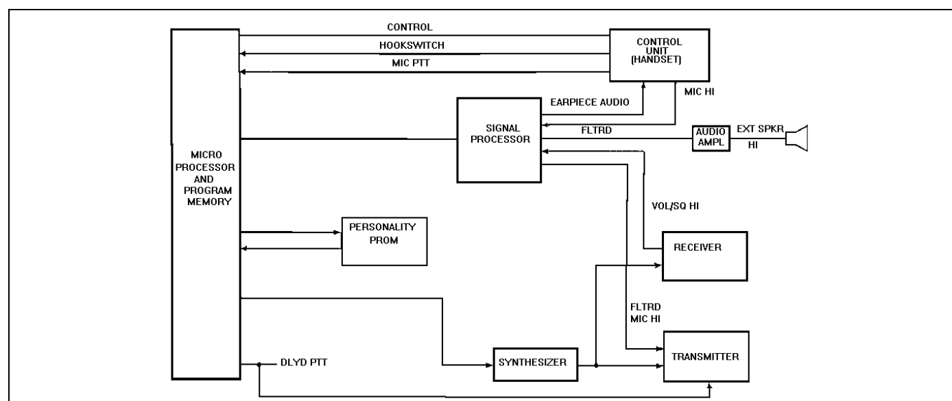
Figure 1 - GE-MARC VE Block Diagram
