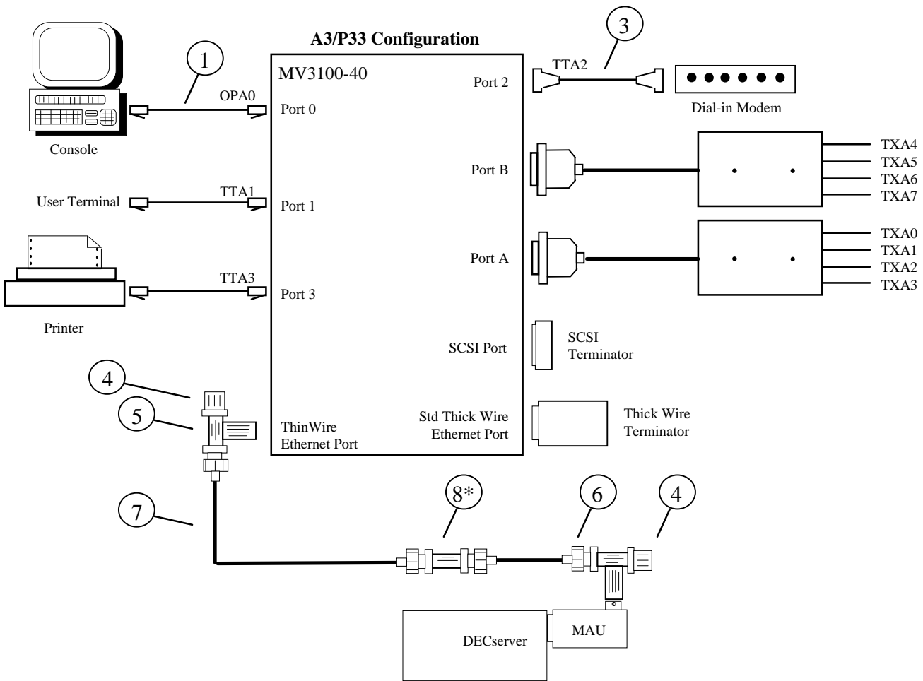
Figure 2-5. Typical A3/P33 System Configuration
