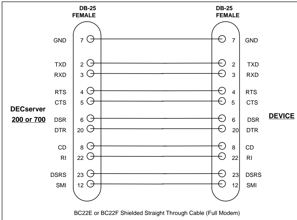
Figure 2-9. Standard System Direct Connect Cable (RS-232)
