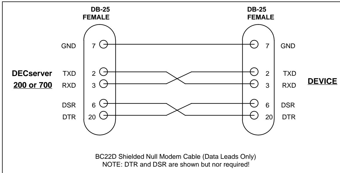
Figure 2-8. Standard System Direct Connect Cable (RS-232)
