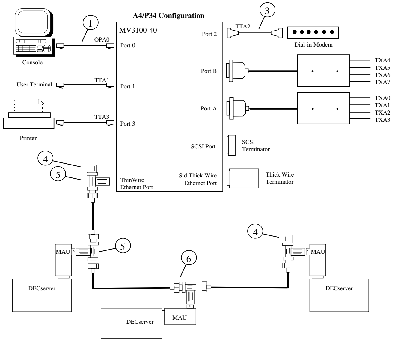
Figure 2-6. Typical A4/P34 System Configuration
