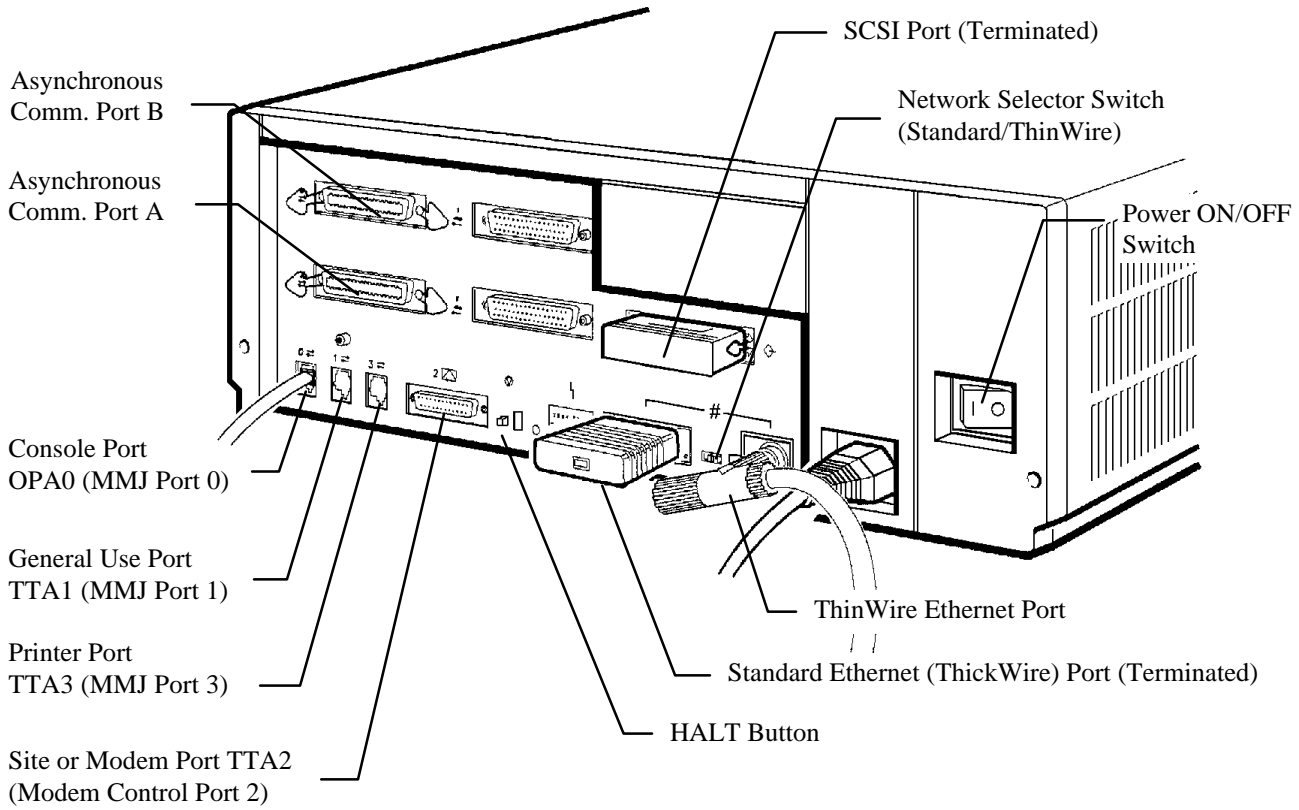
Figure 1-1. System Manager CPU Cabinet (Rear View)
