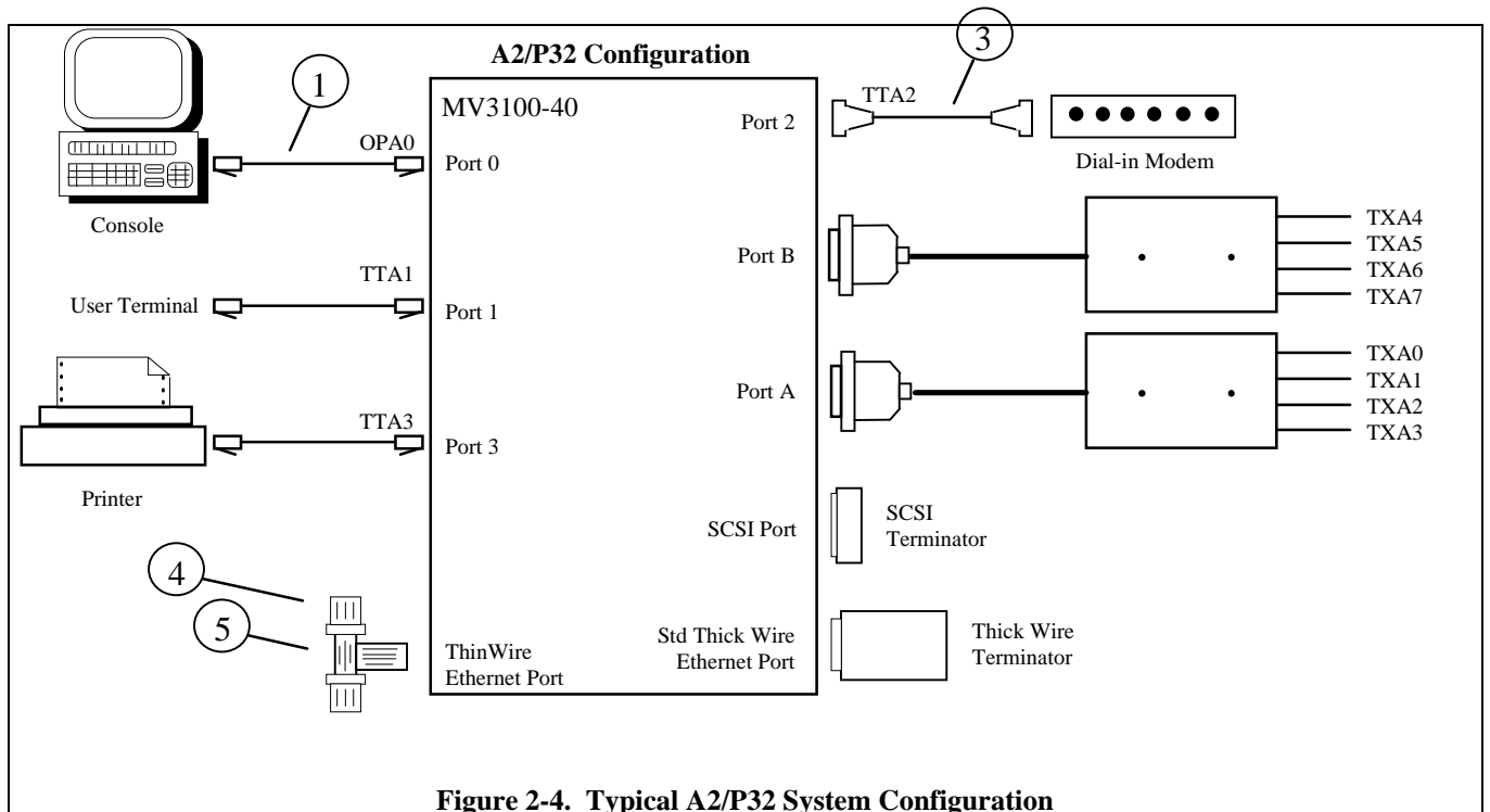
Figure 2-4. Typical A2/P32 System Configuration
