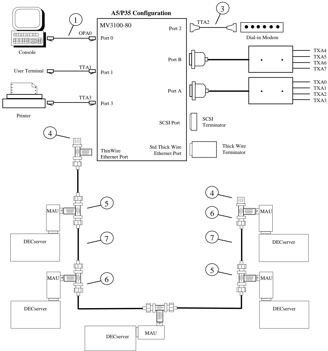
Figure 2-7. Typical A5/P35 System Configuration
