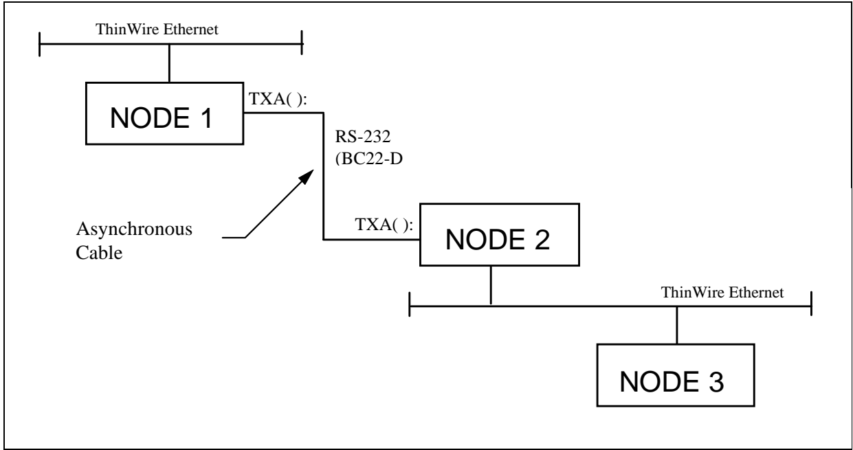
Figure 4-1. Typical Asynchronous DECnet Configuration
