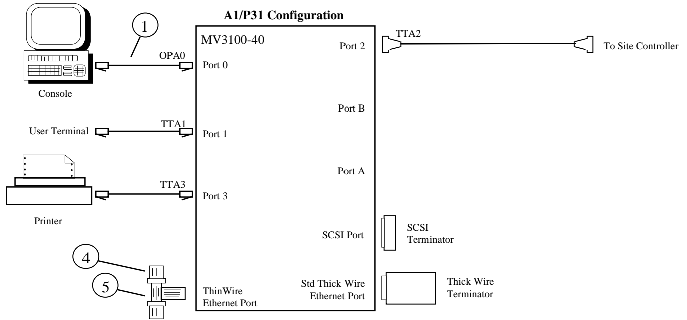
Figure 2-3. Typical A1/P31 System Configuration
