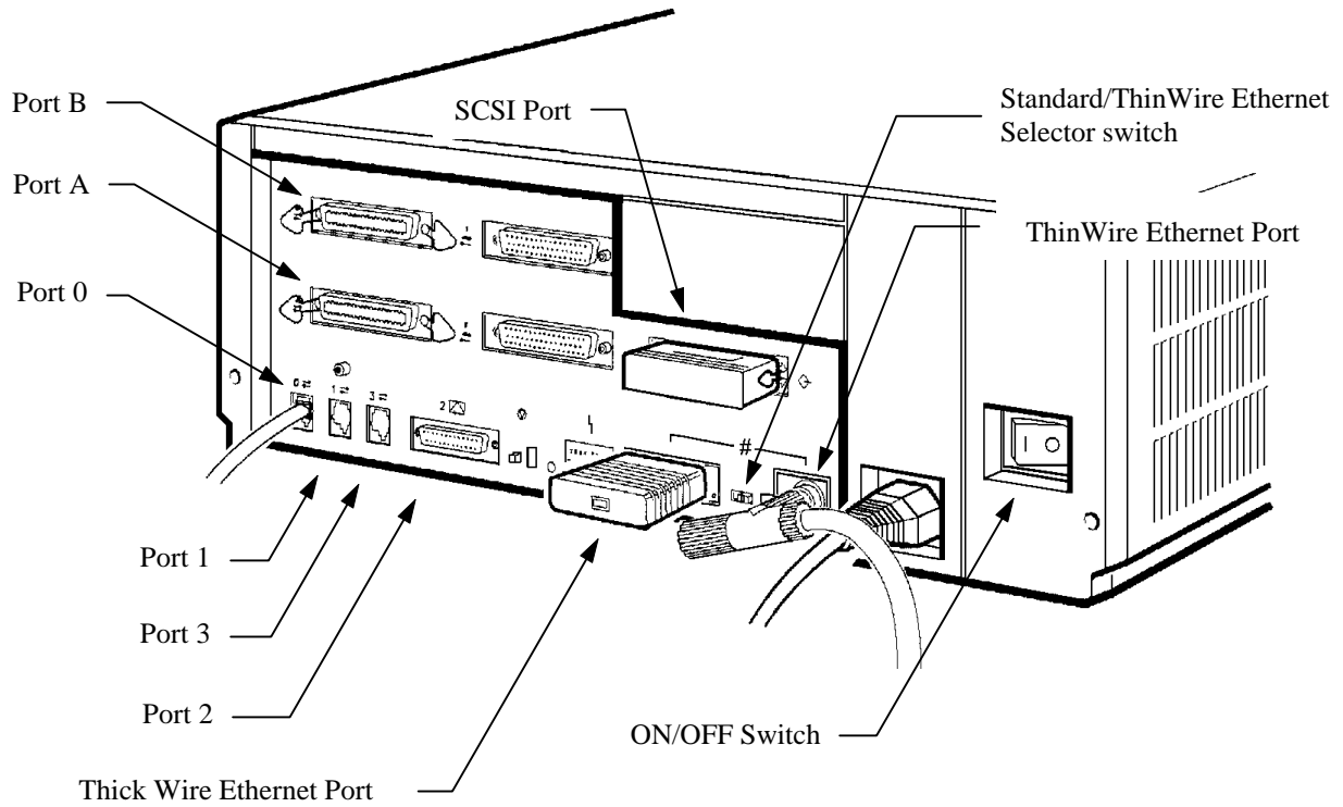
Figure 2-1. MicroVAX I/O Port Diagram:
