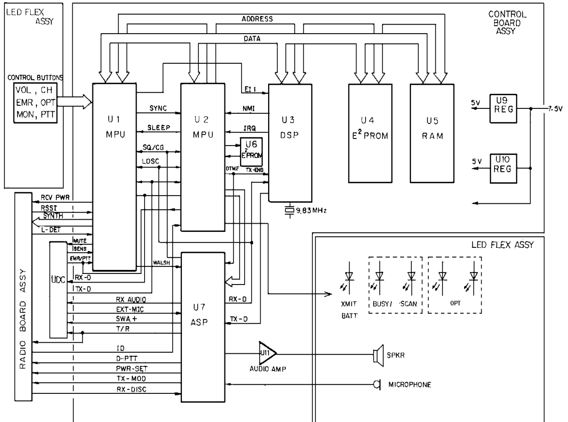
Figure 4 - M-RK I Logic Block Diagram
