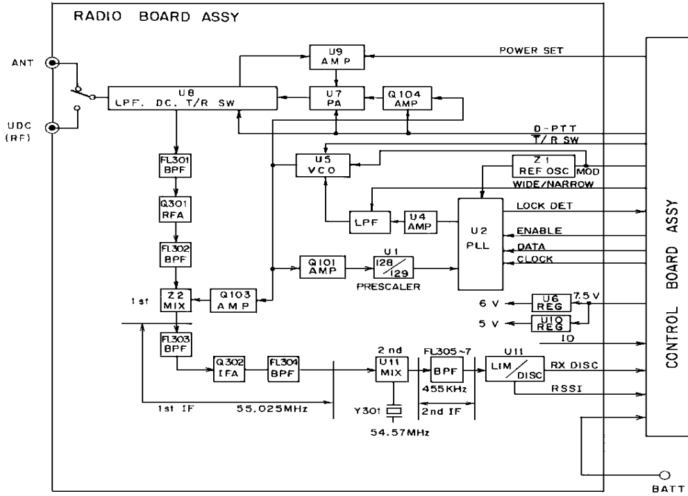
Figure 3 - Radio Block Diagram VHF/UHF
