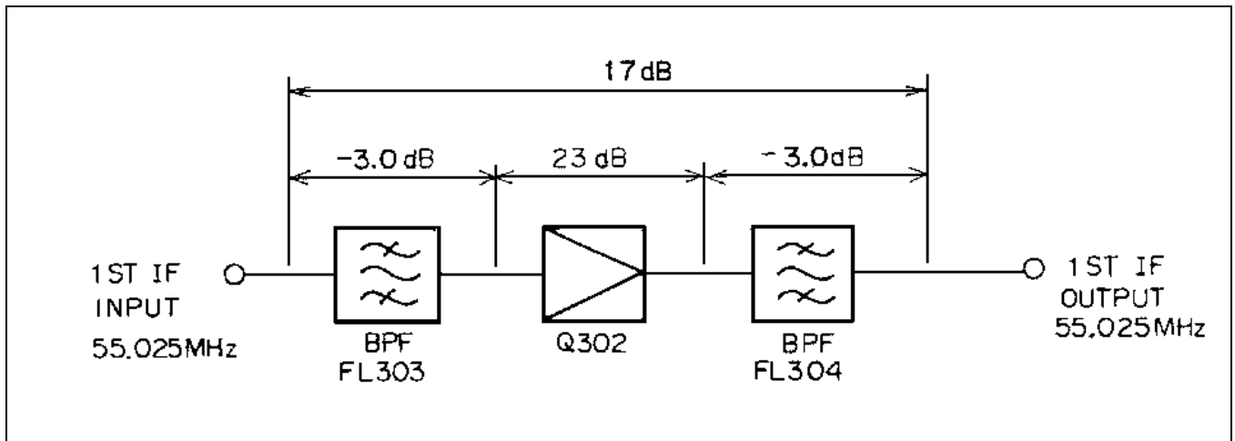
Figure 9 - First IF Amplifier
