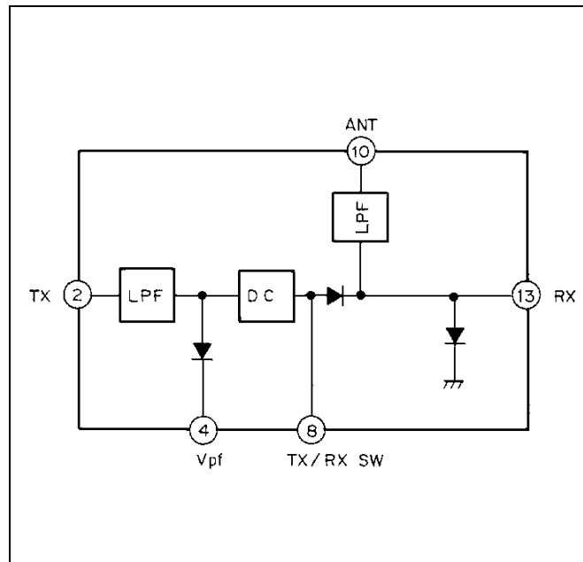
Figure 7 - LPF/DC/T/R SW. Module (U8) VHF/UHF
