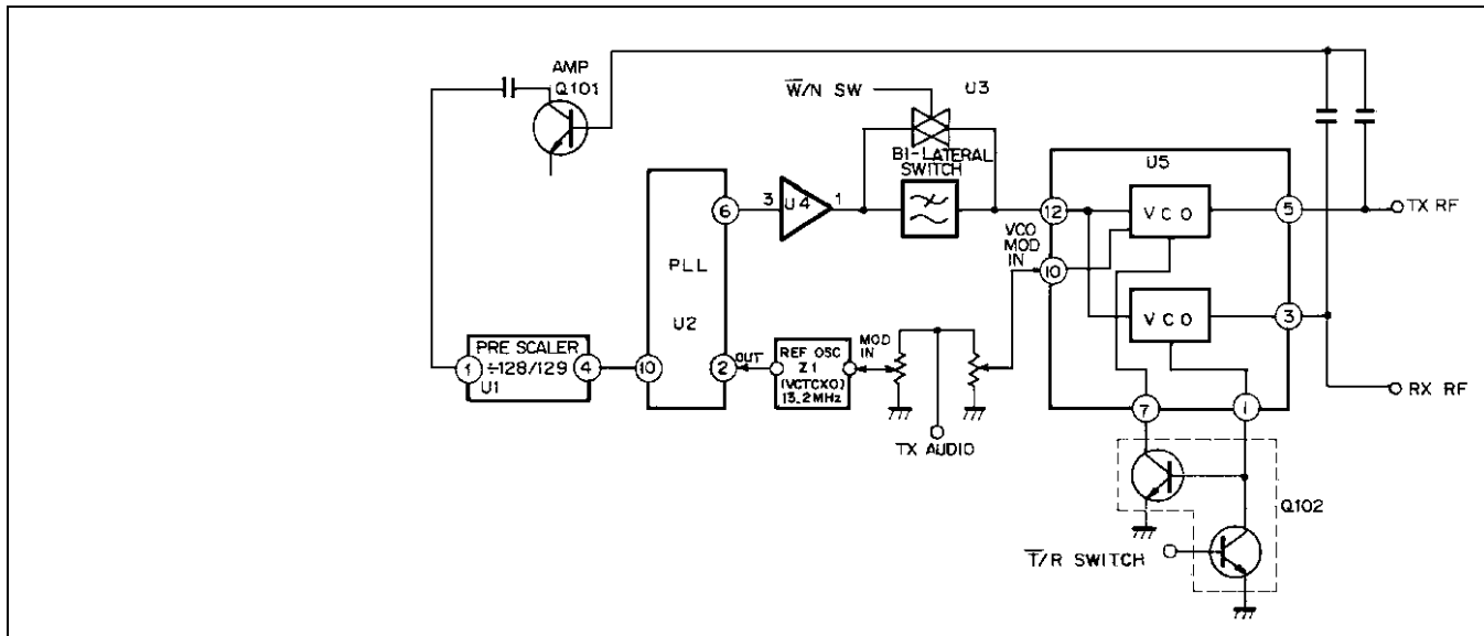
Figure 11 - Synthesizer
