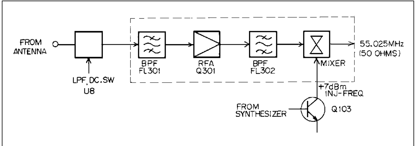
Figure 8 - RF Amplifier/Mixer
