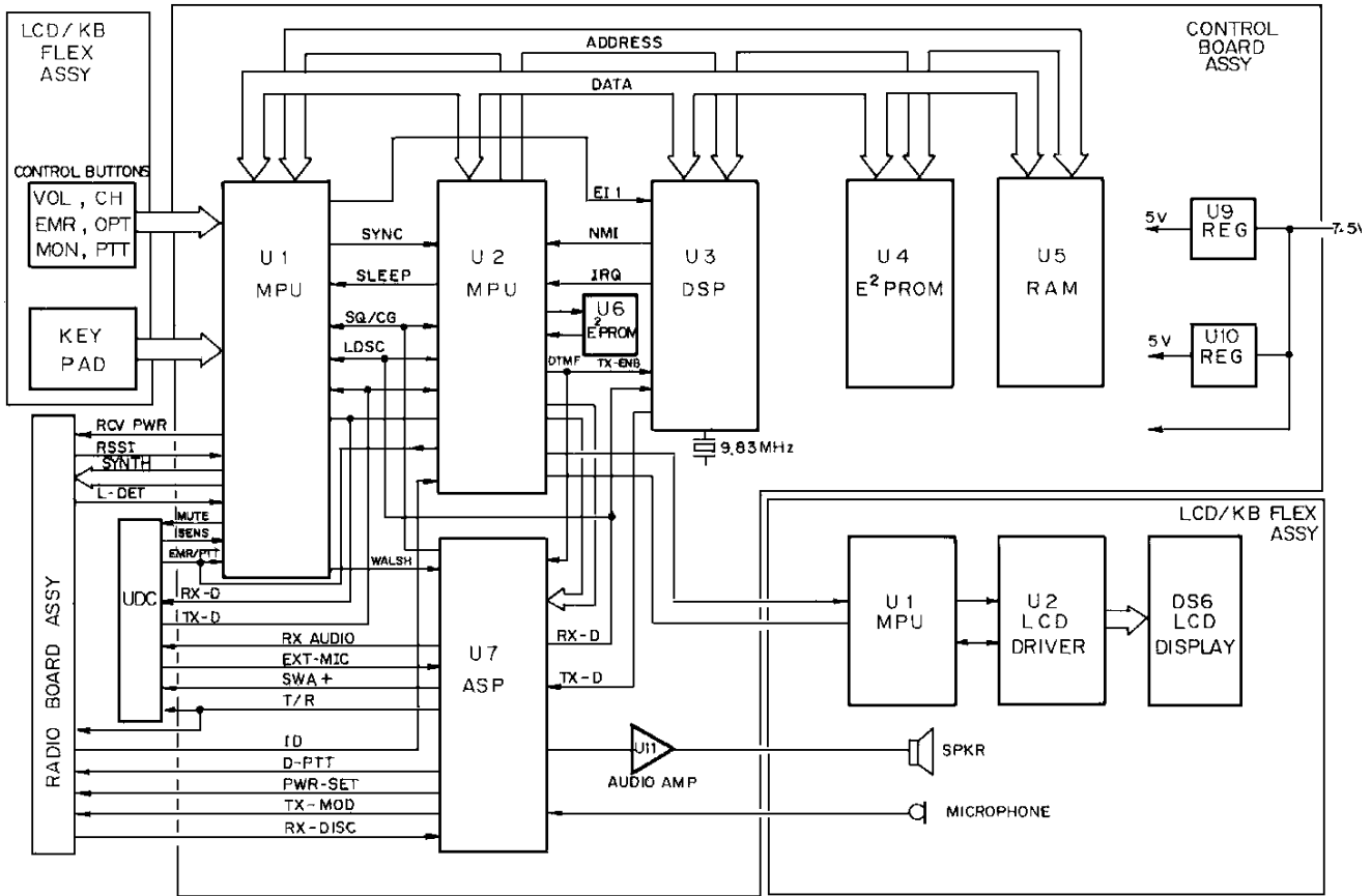
Figure 5 - M-RK II & Scan Logic Block Diagram
