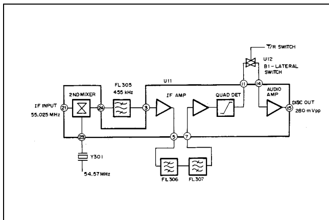
Figure 9 - Second IF Amplifier/Discriminator
