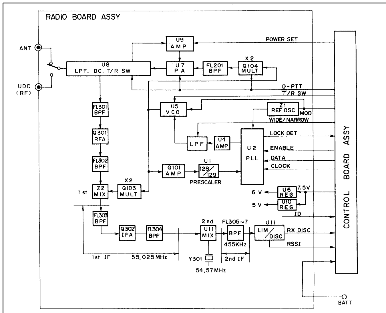
Figure 3 - Radio Block Diagram
