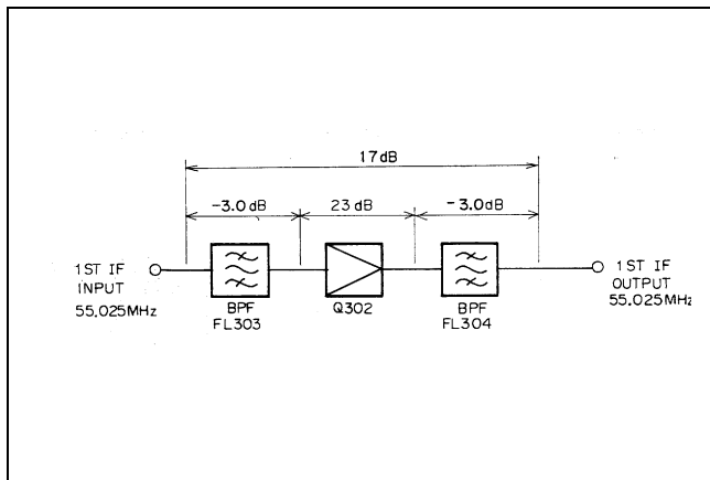
Figure 8 - First IF Amplifier
