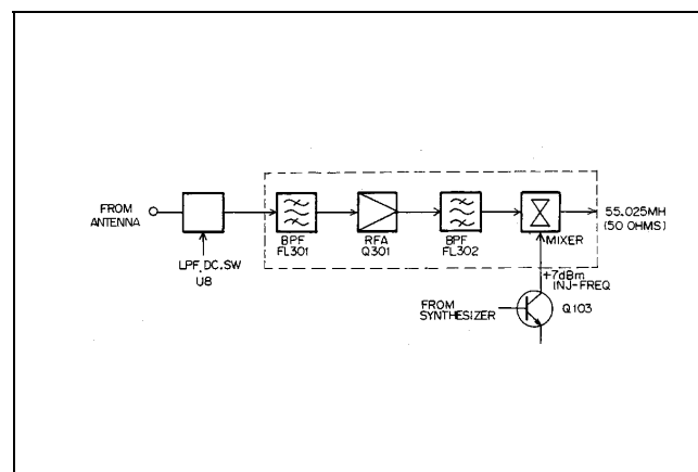
Figure 7 - RF Amplifier/Mixer
