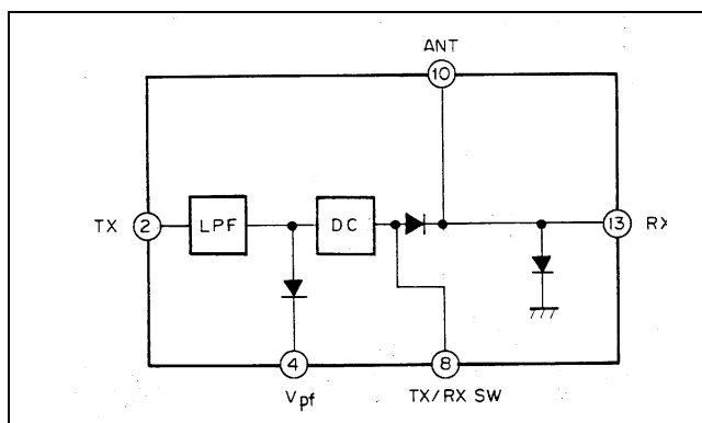
Figure 6 - LPF, DC, T/R SW. Module (U8)
