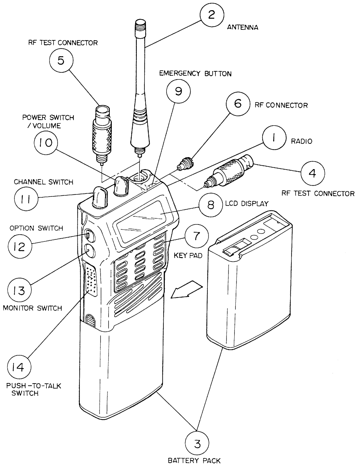
Figure 2 - M-RK II Controls and Accessories
