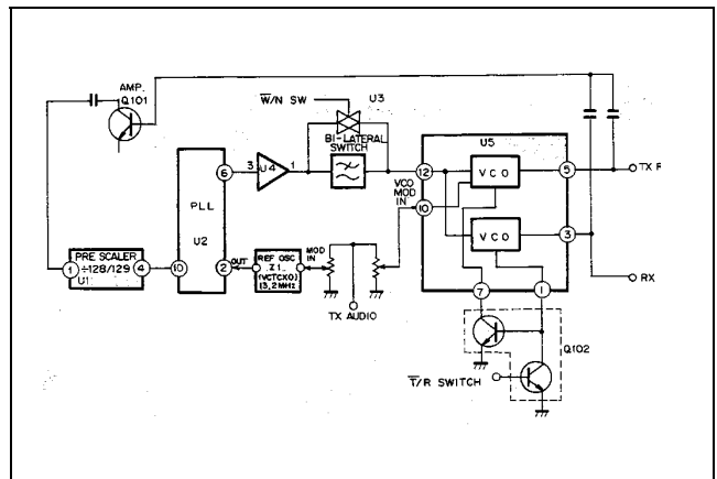
Figure 10 - Synthesizer
