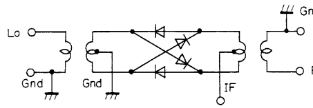
RF BOARD DOUBLE BALANCED DIODE MIXER (DBM) (Z2)
