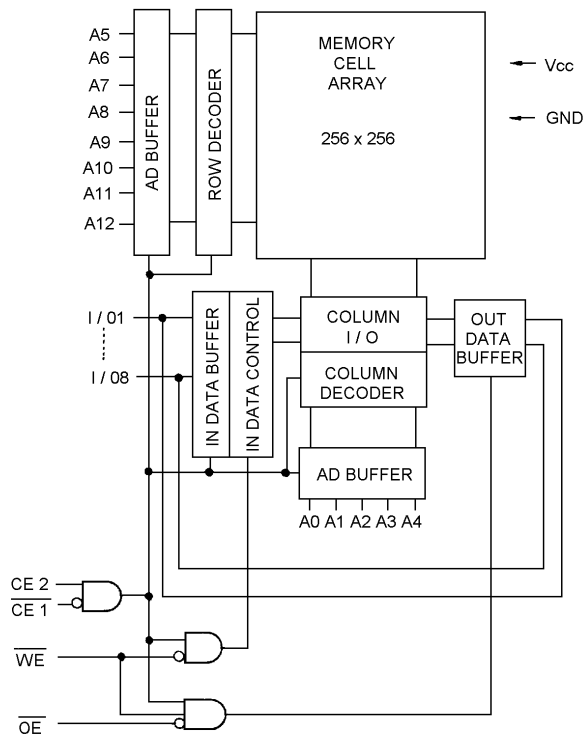
BLOCK DIAGRAM
