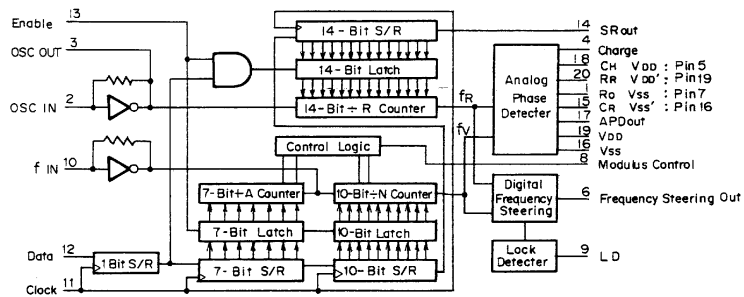
BLOCK DIAGRAM
