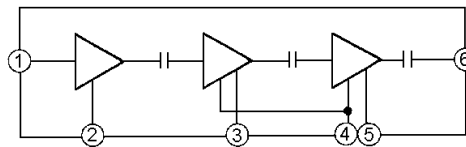
INTERNAL DIAGRAM
