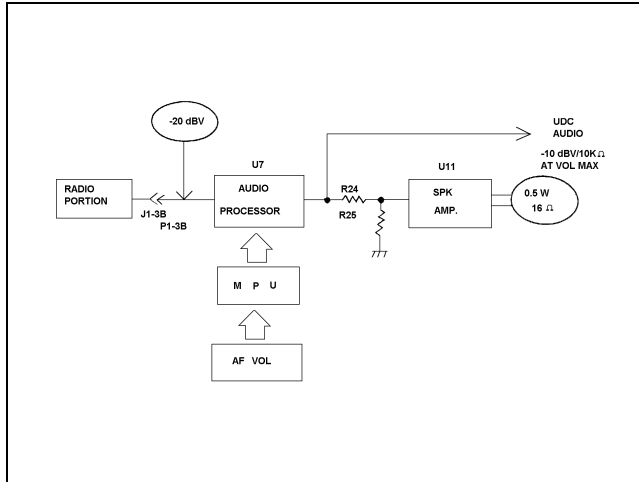
Figure 6 - Receiver Audio Output
