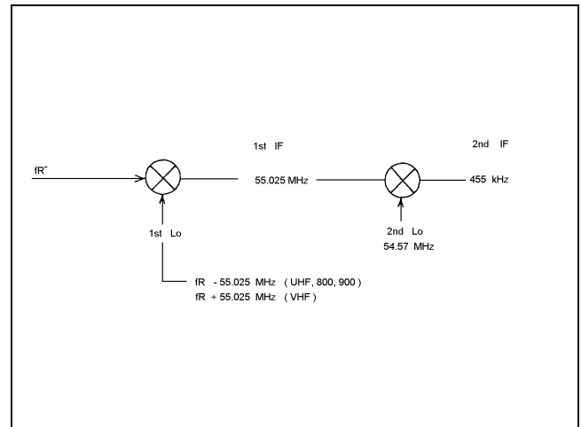
Figure 7 - Frequency Relationship Diagram
