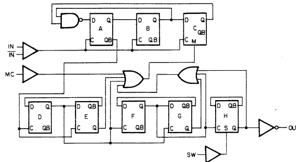
BLOCK DIAGRAM
