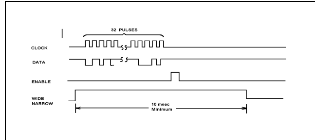
Figure 2 - Clock, Data, Enable, And Wide/Narrow Signals
