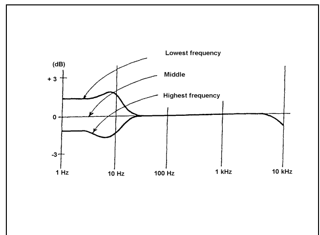
Figure 5 - Typical Frequency Characteristics
