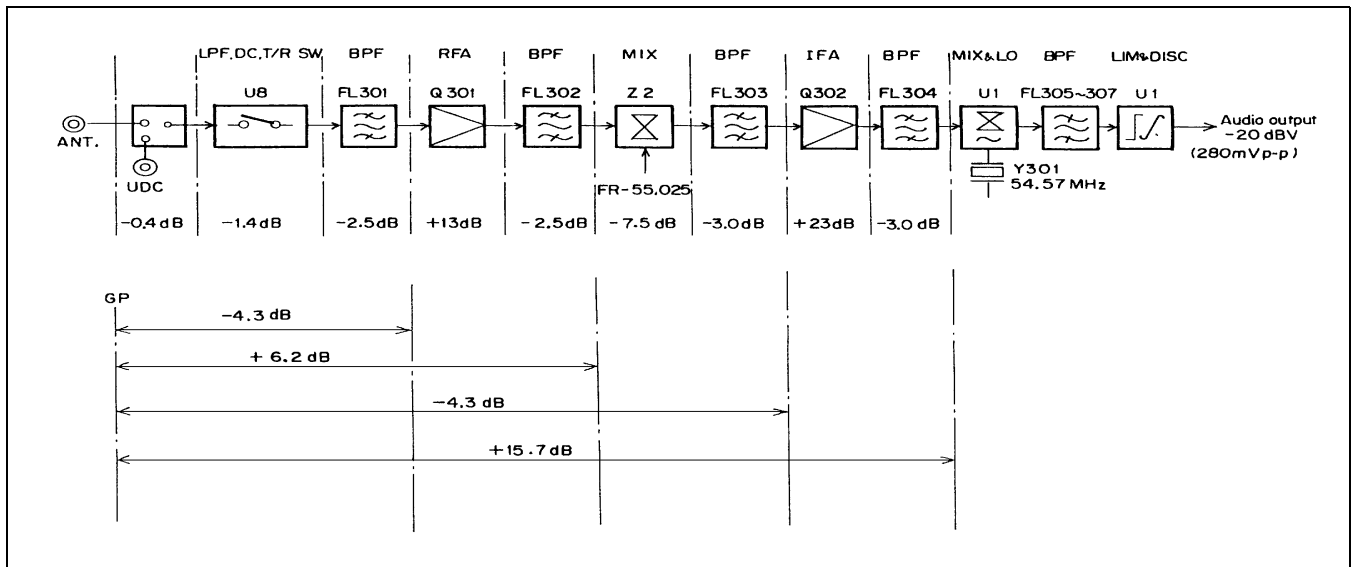
Figure 8 - Typical Level Diagram
