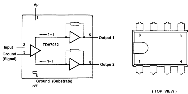
BLOCK DIAGRAM
