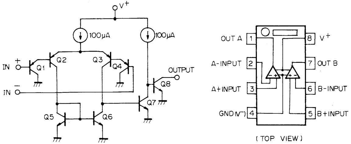
Equivalent Circuit (1/2 Circuit)
