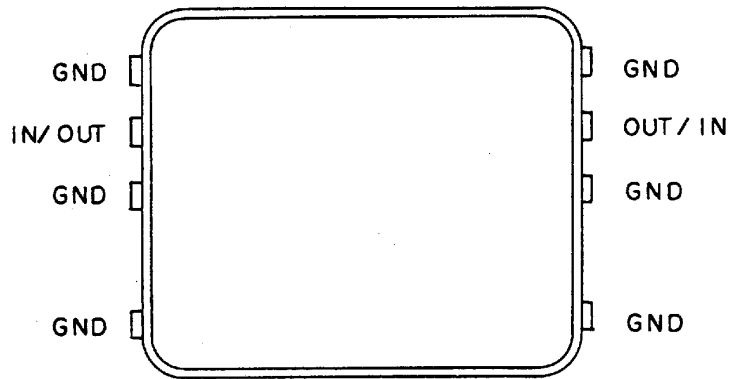
UHF ( TOP VIEW )
