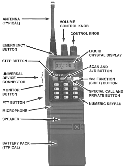
Figure 1 - Aegis EDACS M-PA System Model Radio
