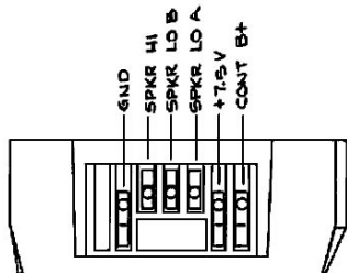
BATTERY CONTACT IDENTIFICATION VIEWED FROM OUTSIDE OF CASE
