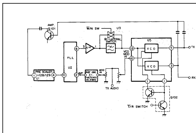
Figure 11 - Synthesizer
