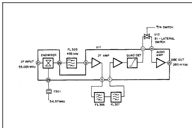
Figure 10 - Second IF Amplifier/Discriminator
