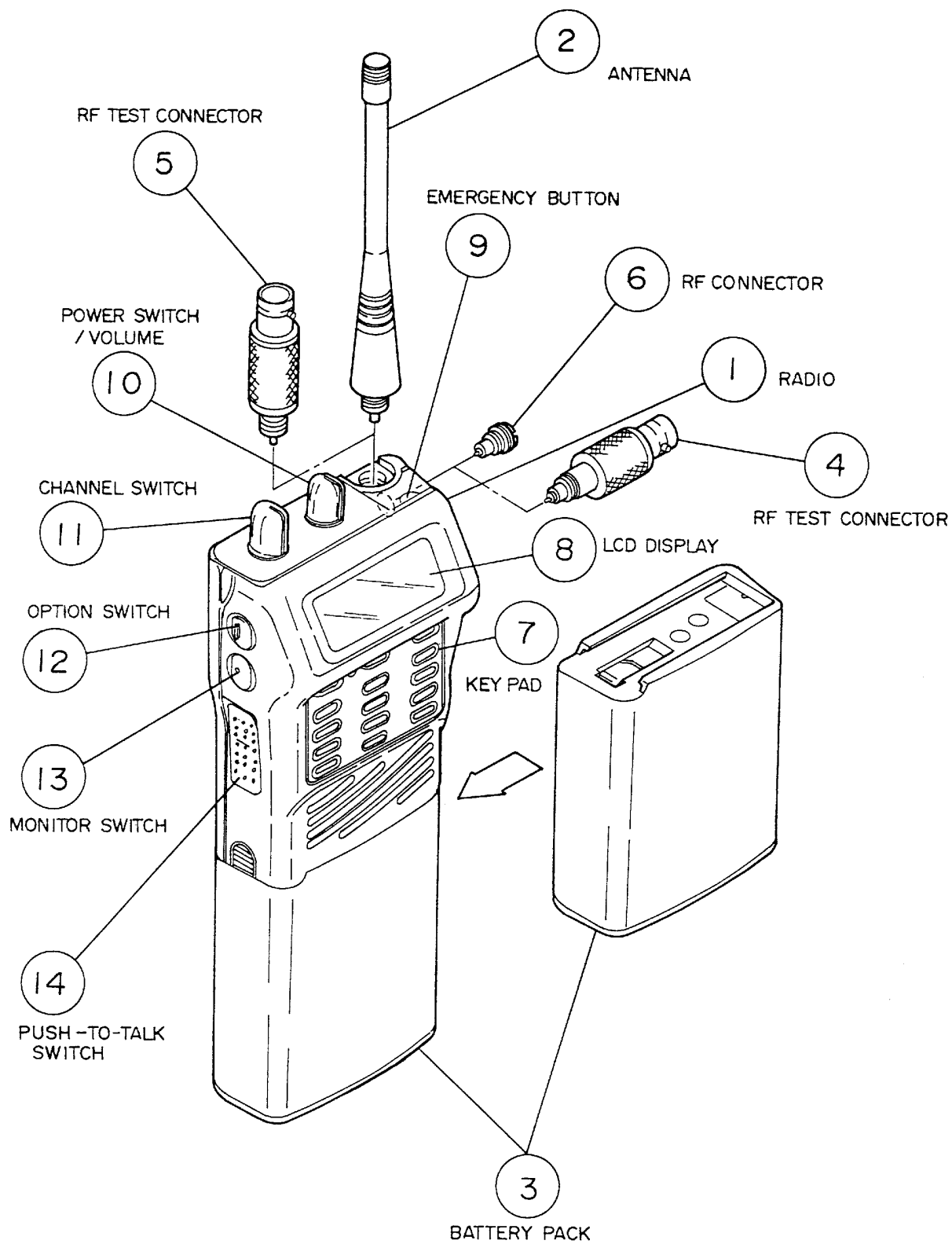
Figure 2 - M-RK II Controls and Accessories
