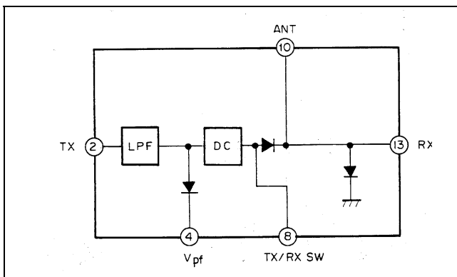
Figure 7 - LPF DC T/R SW. Module (U8)
