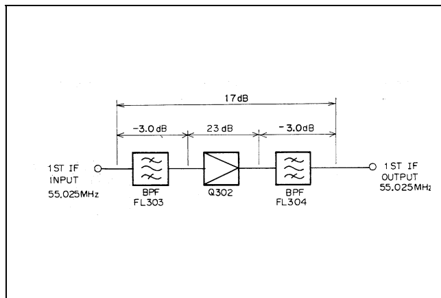
Figure 9 - First IF Amplifier
