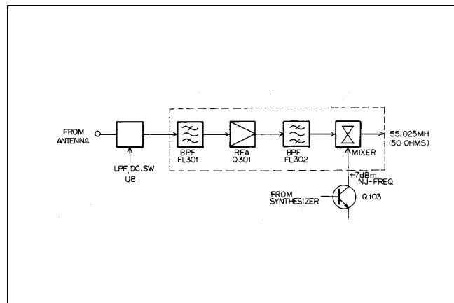
Figure 8 - RF Amplifier/Mixer
