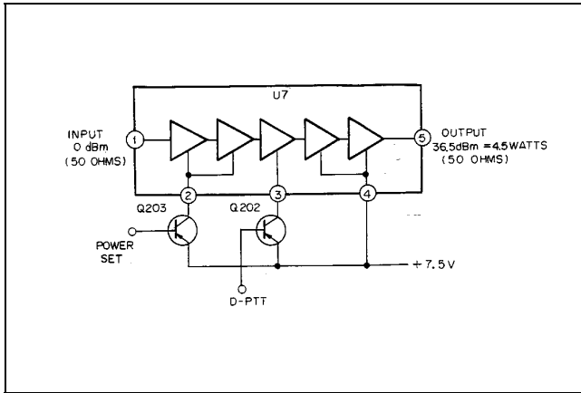
Figure 6 - Power Amplifier (PA)
