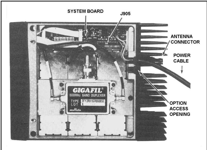
Figure 10 - Bottom View (Cover Removed)
