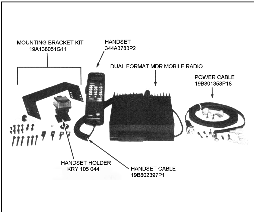
Figure 1 - Dual Format MDR Mobile Radio Components and Mounting Hardware
