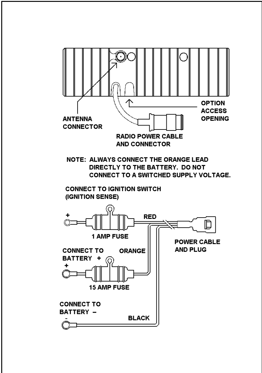
Figure 3 - Power Cable
