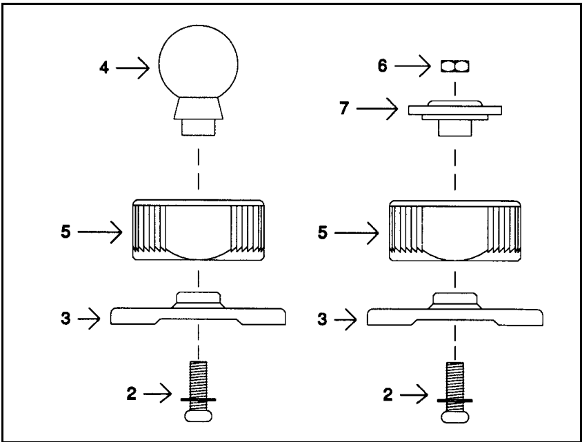
Figure 7 - Handset Holder Base Breakdown
