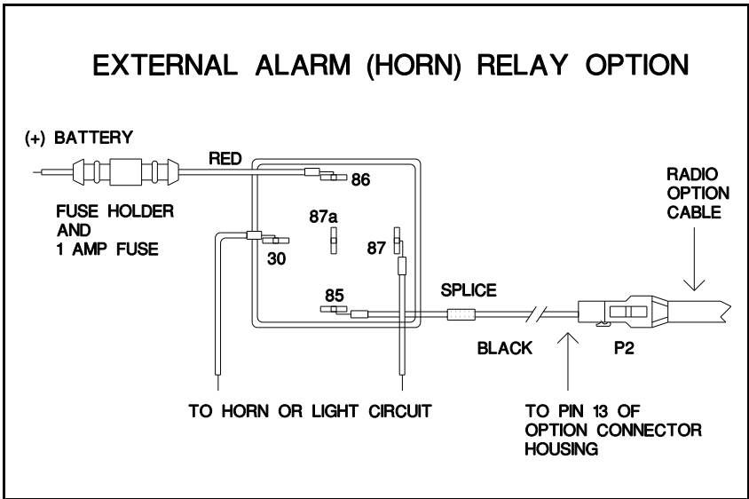
Figure 11 - External Alarm Relay
