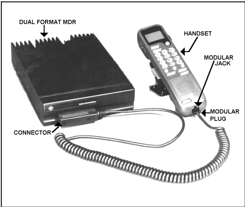
Figure 8 - Dual Format MDR Mobile Radio With Handset And Cable
