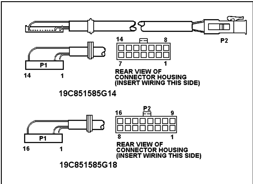
Figure 9- Option Cable Pin Locations
