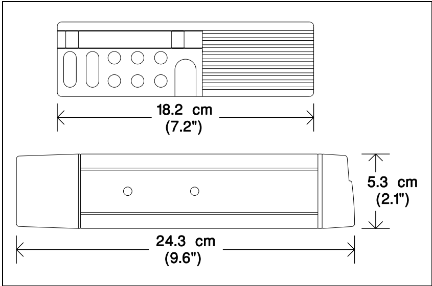
Figure 4 - Mounting Dimensions
