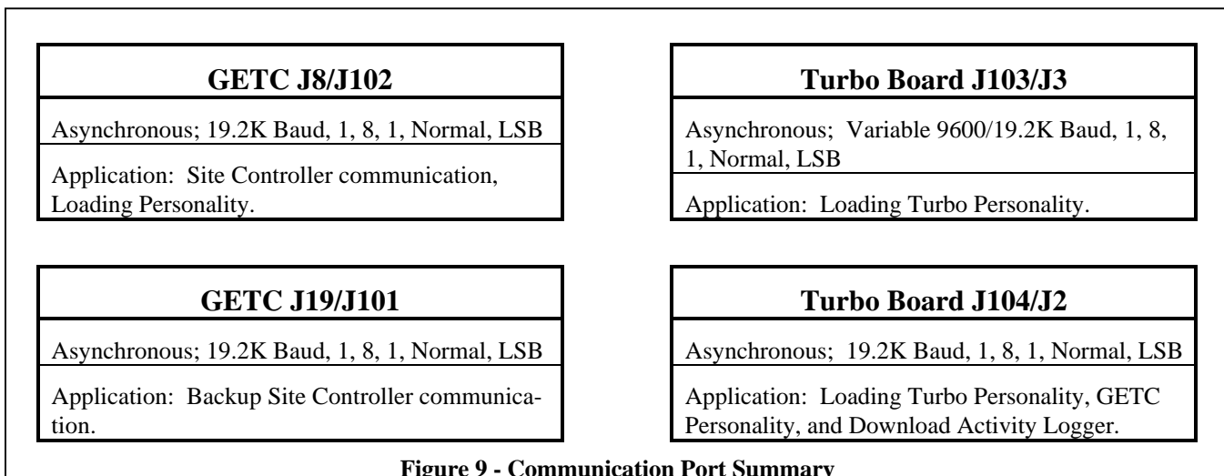
Figure 9 - Communication Port Summary
