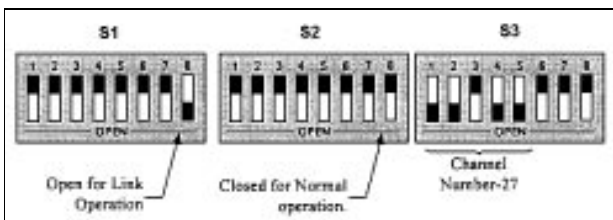
Figure 8 - Operational DIP Switch Settings For DL Set To Channel 27
