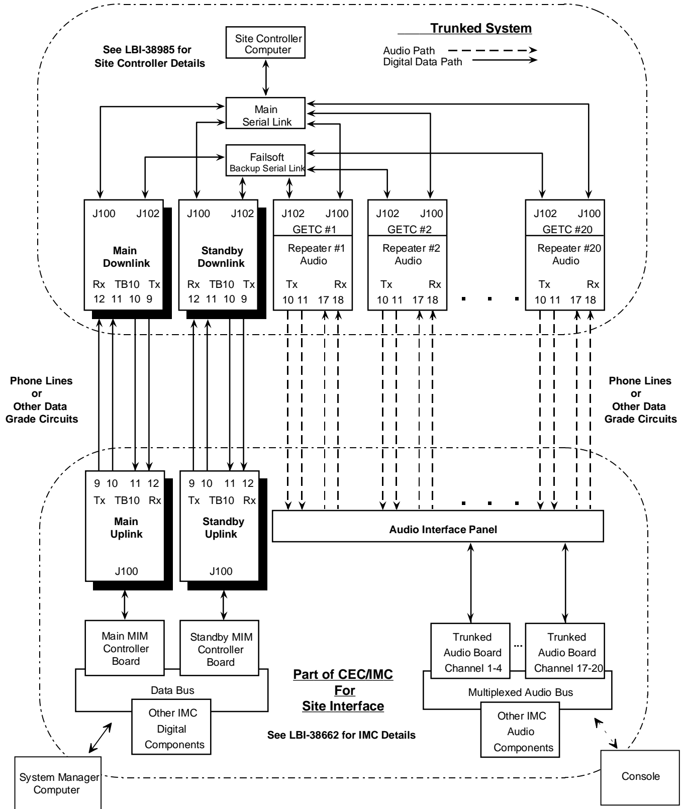
Figure 1 - Downlink and the CEC/IMC's Uplink for a Single Site Trunked System
