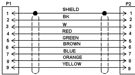
CONNECTION DIAG
