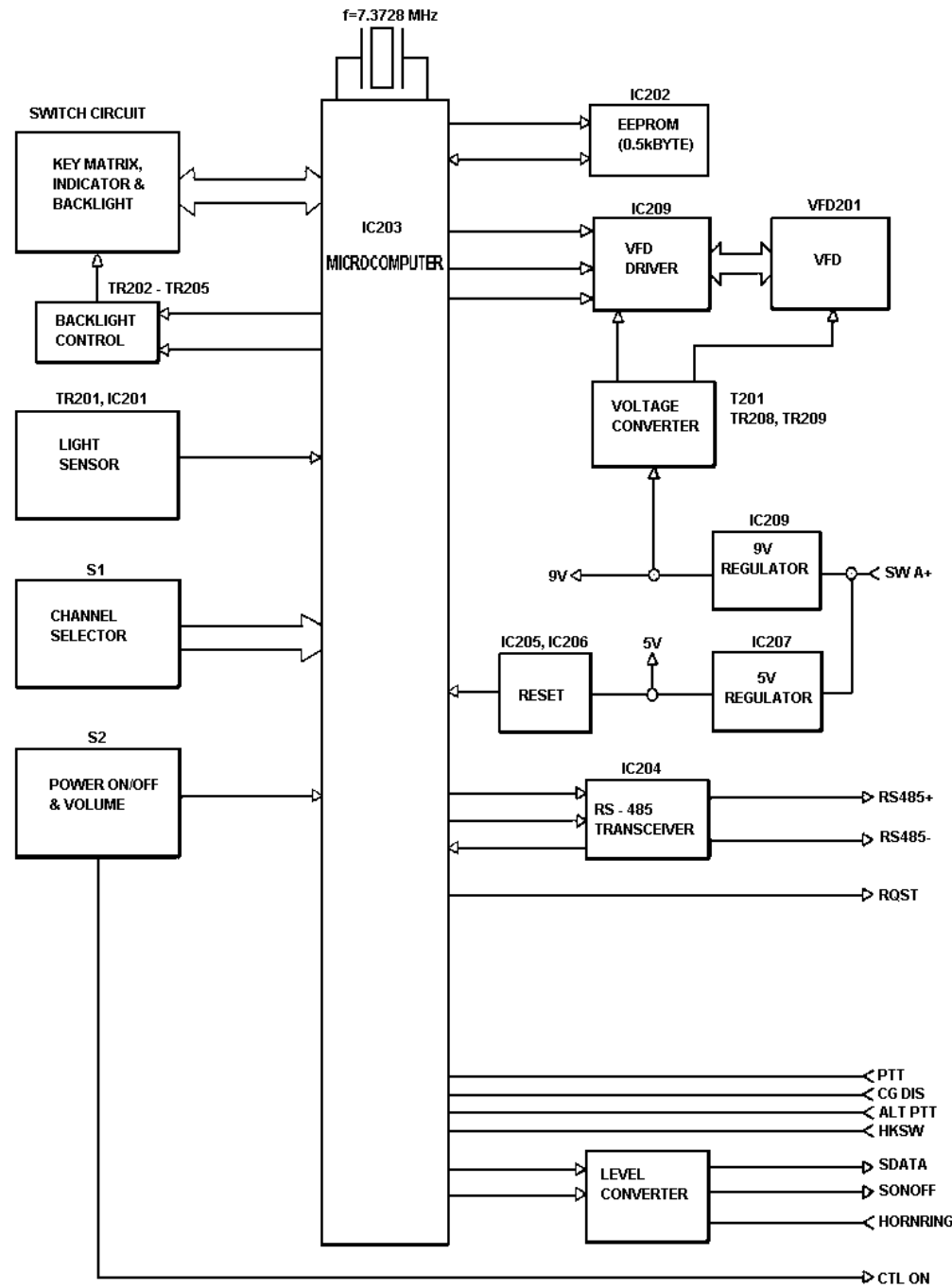
Figure 3 - Block Diagram
