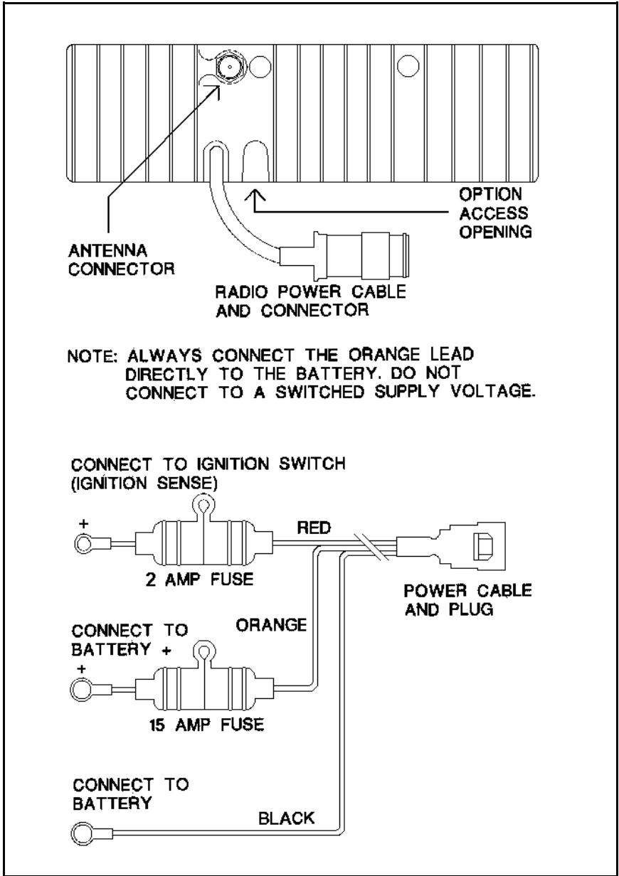
Figure 3 - Power Cable
