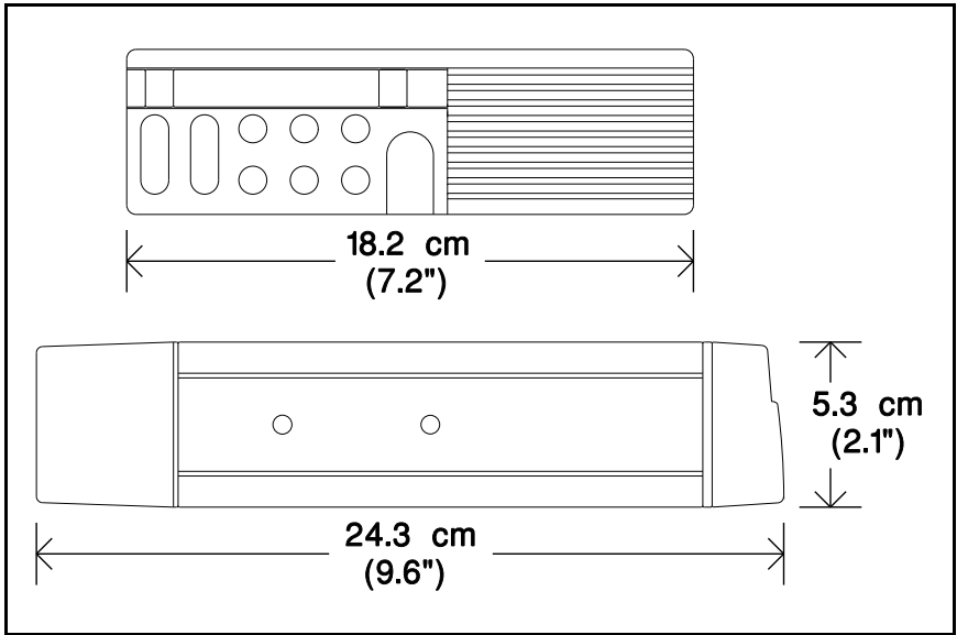
Figure 4 - Mounting Dimensions
