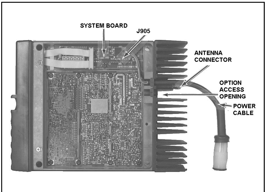
Figure 11 - Bottom View (Cover Removed)
