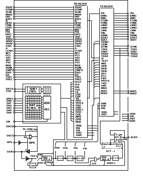
BLOCK DIAGRAM
