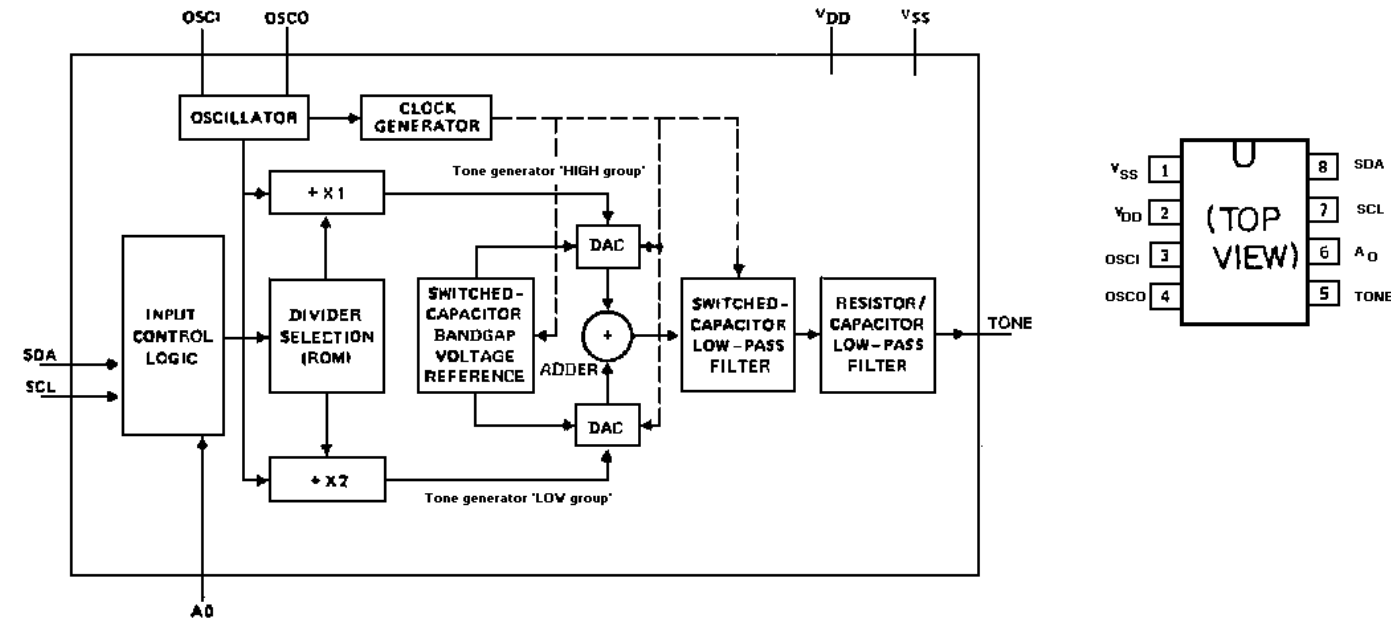
BLOCK DIAGRAM
