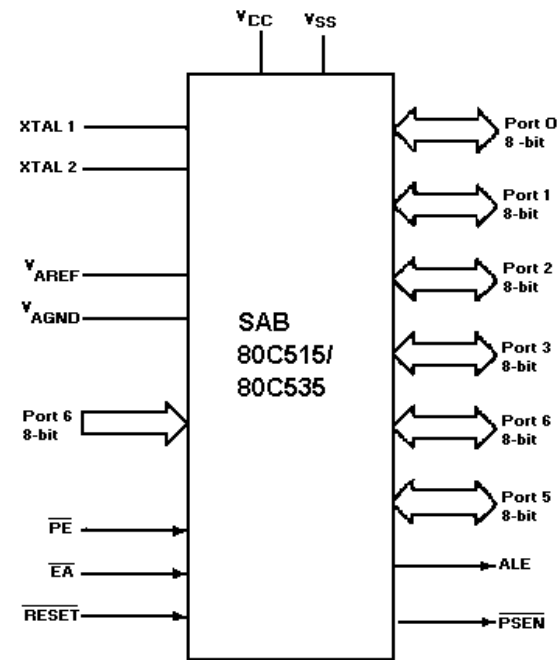
Logic Symbol
