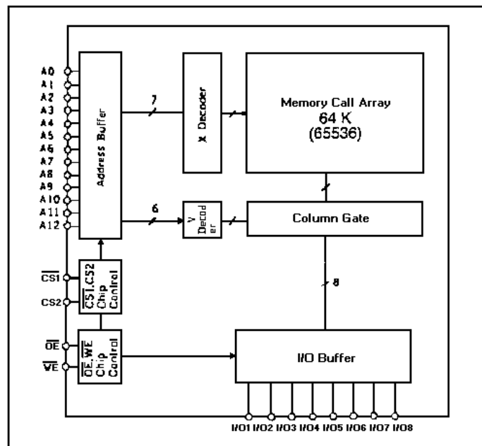
BLOCK DIAGRAM
