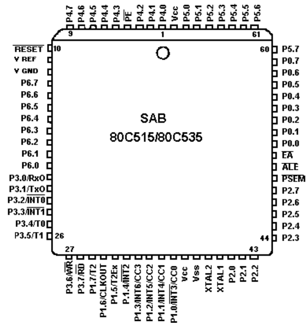
Pin Configuration PL-CC-68
