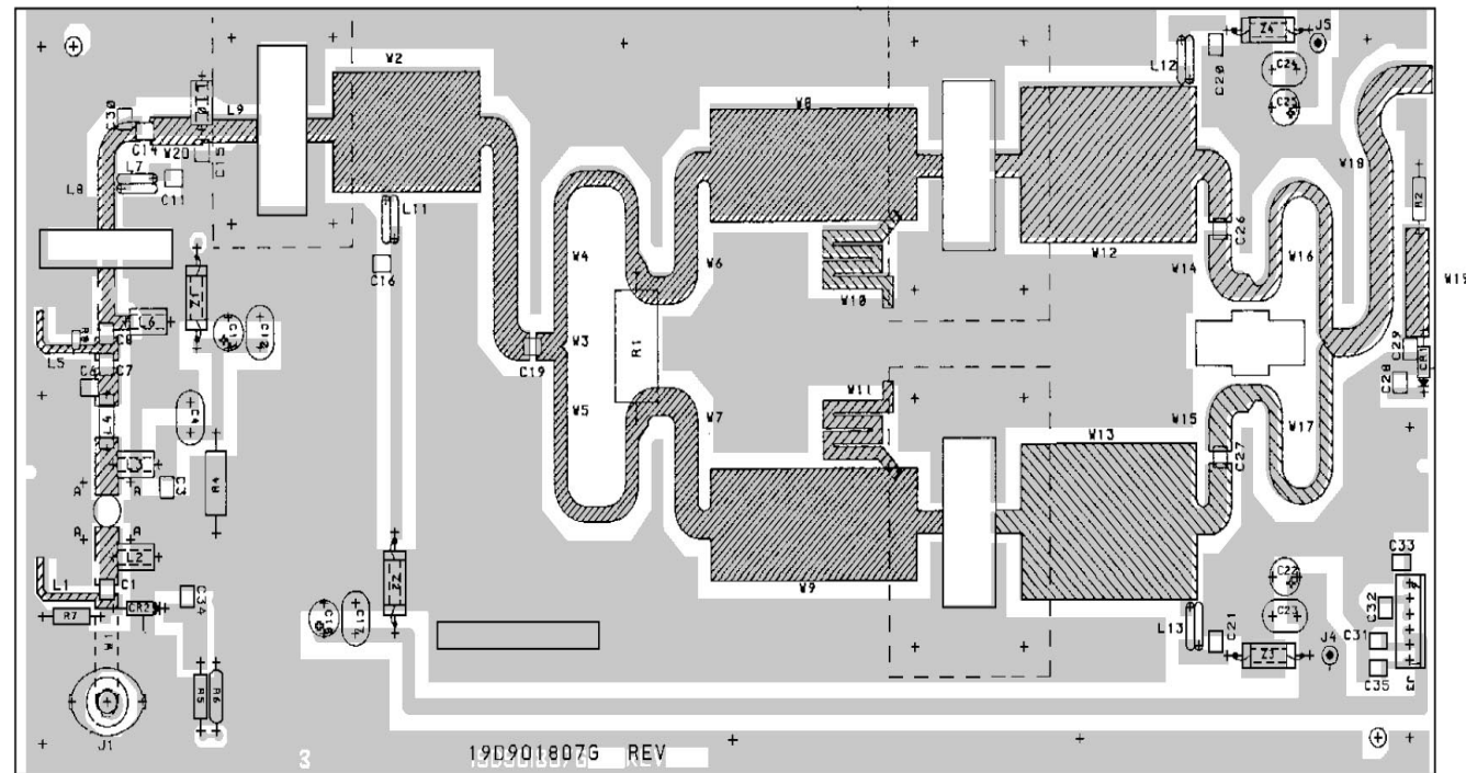
COMPONENT SIDE
