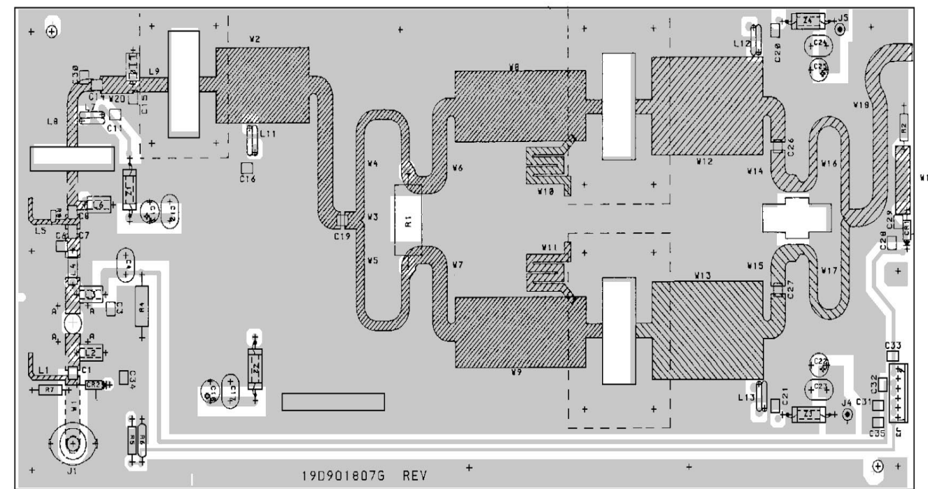
SOLDER SIDE
