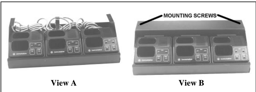
Figure 2 - Assembly Instructions
