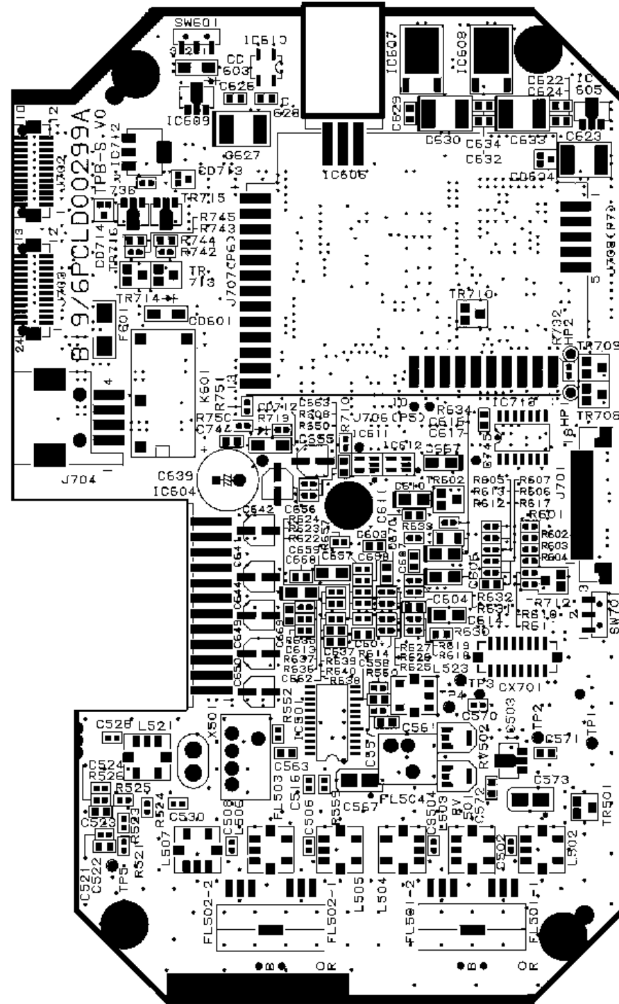
COMPONENT SIDE
