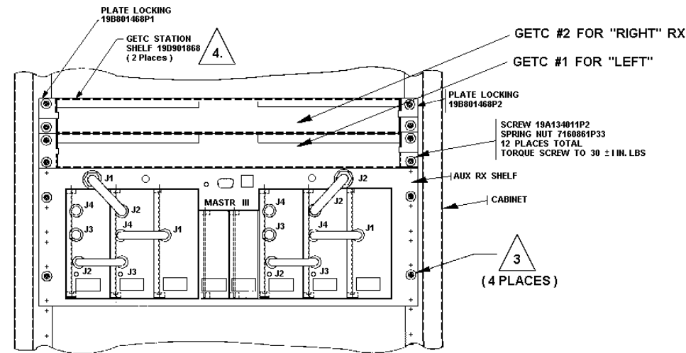
PARTIAL FRONT VIEW OF CABINET
