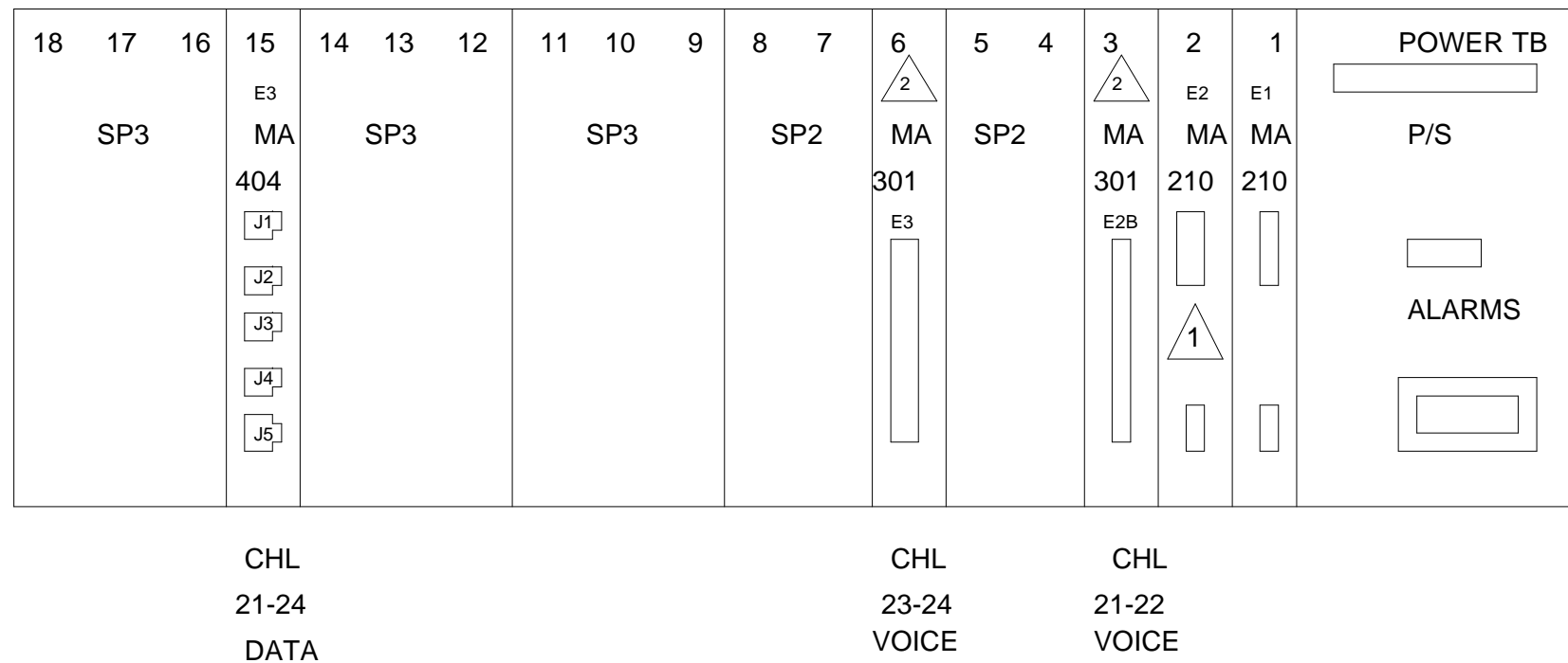
INTRAPLEX TDM-163 EXPANSION SHELF (24 Chan Config.) [5 Time Slots]
