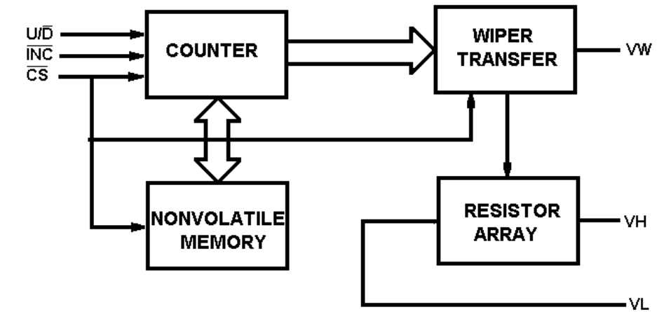
Potentiometer, Digitally Controlled U121, U321 19A705180P2 (X9103)
