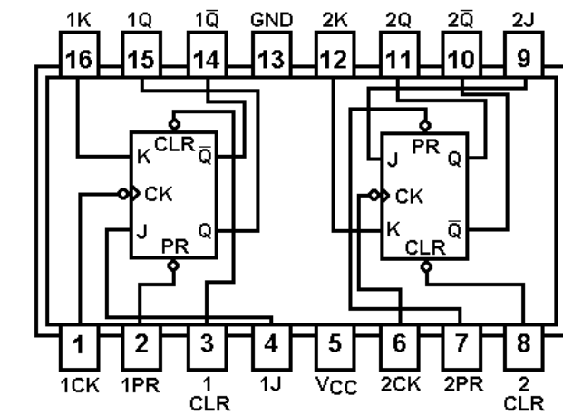
Dual J-K Flip-Flop with Preset and Clear U202 19A700037P337 (74LS76A)
