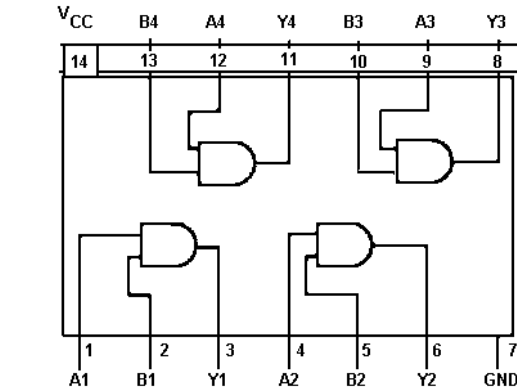
Dual 2-Input, Positive AND gate U315, U403 19A700037P307 (74LS08)
