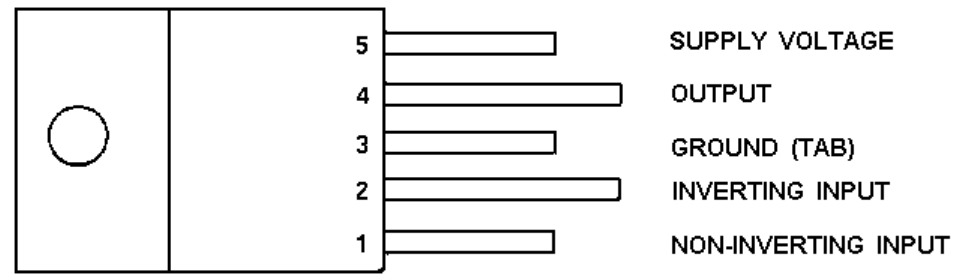
PIN IDENTIFICATION
