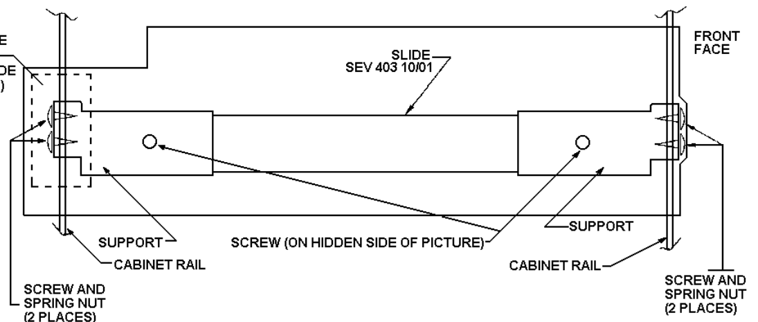
DETAIL - 1: SUPPORT & SLIDE PLACEMENT
