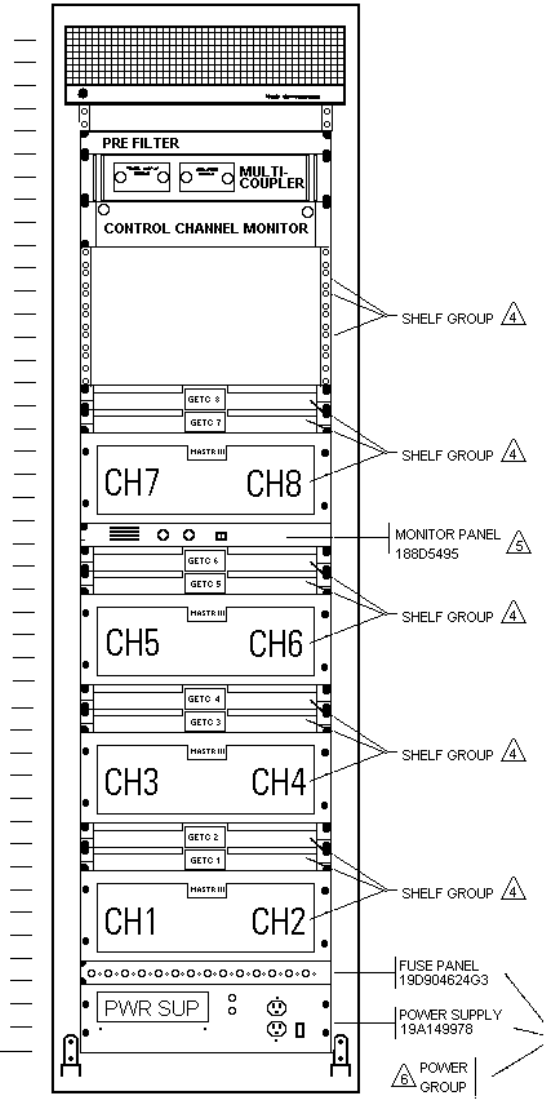
FRONT VIEW (DOORS REMOVED FOR CLARITY)
