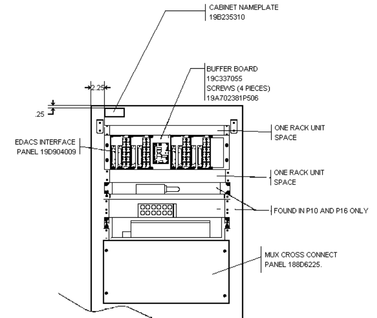
REAR VIEW, TOP OF ALL CABINETS
