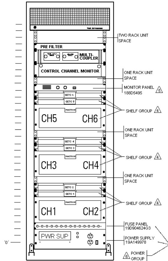
FRONT VIEW
