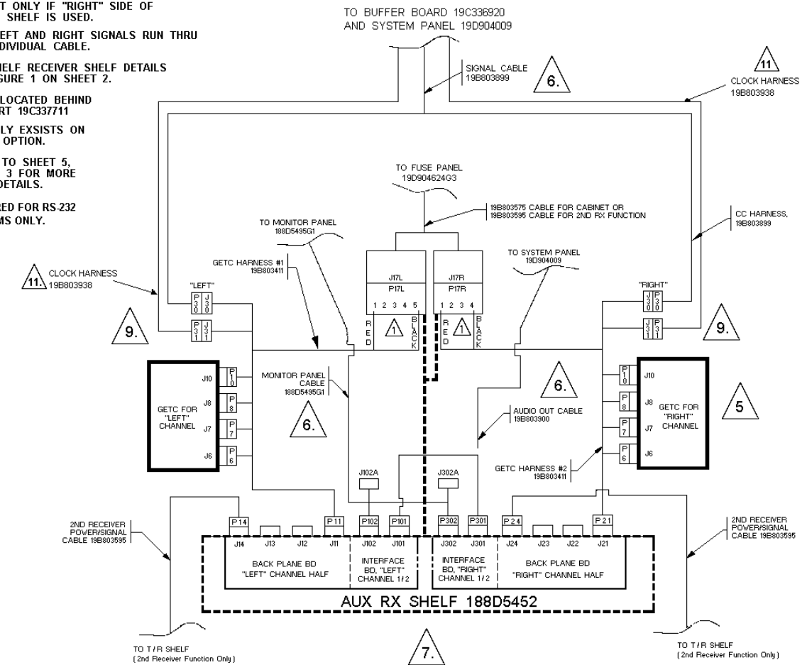
SHELF & GETC CONNECTION DIAGRAM
