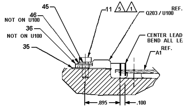
SECTION C - C (TAKEN FROM SHEET 1) LEAD FORMING AND HARDWARE STACKUP FOR Q203 & U100 FOR Q203, U100 USE EGE TOOL #423445G1A
