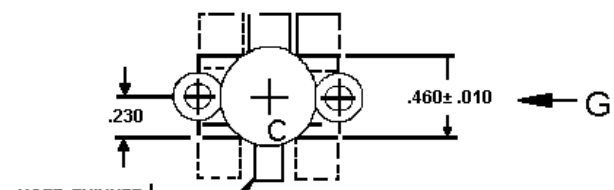
DETAIL F LEAD TRIMMING FOR Q1 THRU Q3 G3 USE EGE TOOL #423445 G1C FOR Q101 THRU Q103, G1 USE EGE TOOL #902/97 -G1A (TAKEN FROM SHEET 1)
