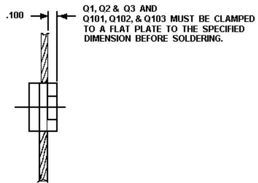
VIEW G TYPICAL LEAD FORMING & ASSEMBLY POSITIONING FOR Q1 THRU Q3 FOR Q101 THRU Q103
