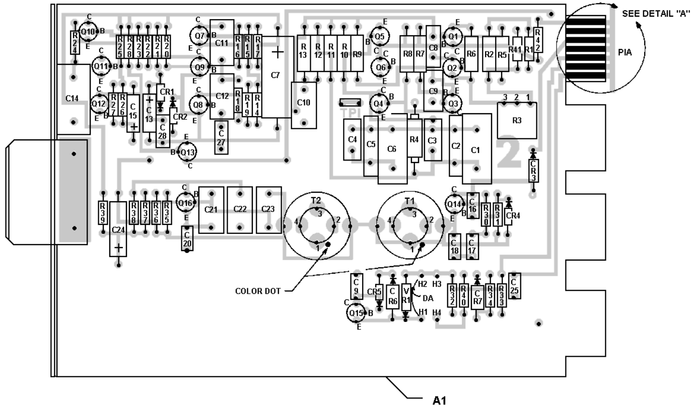
TRANSMIT DETECTOR BOARD 19D417263G1
