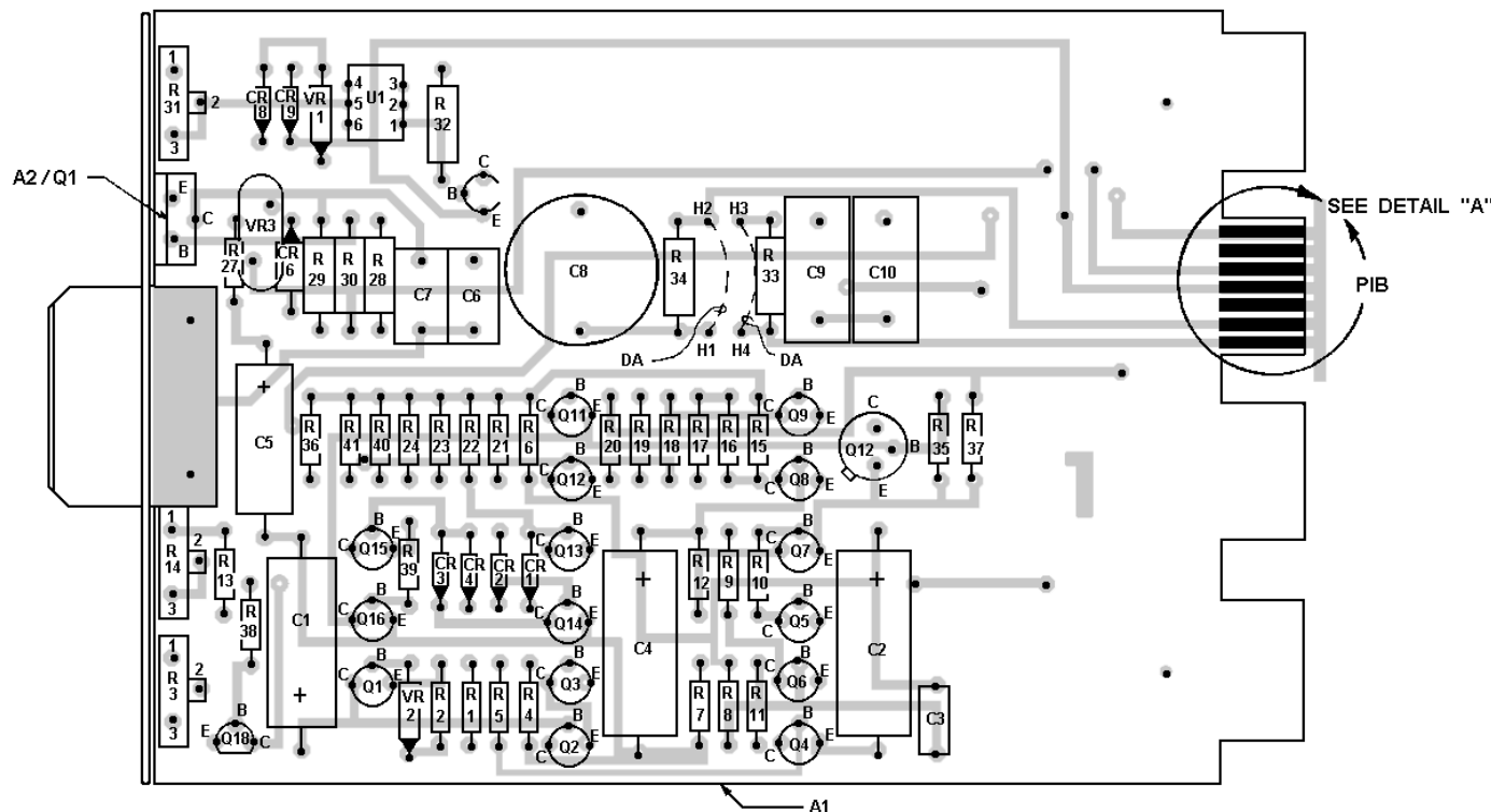
TRANSMIT DETECTOR BOARD 19D417263G1
