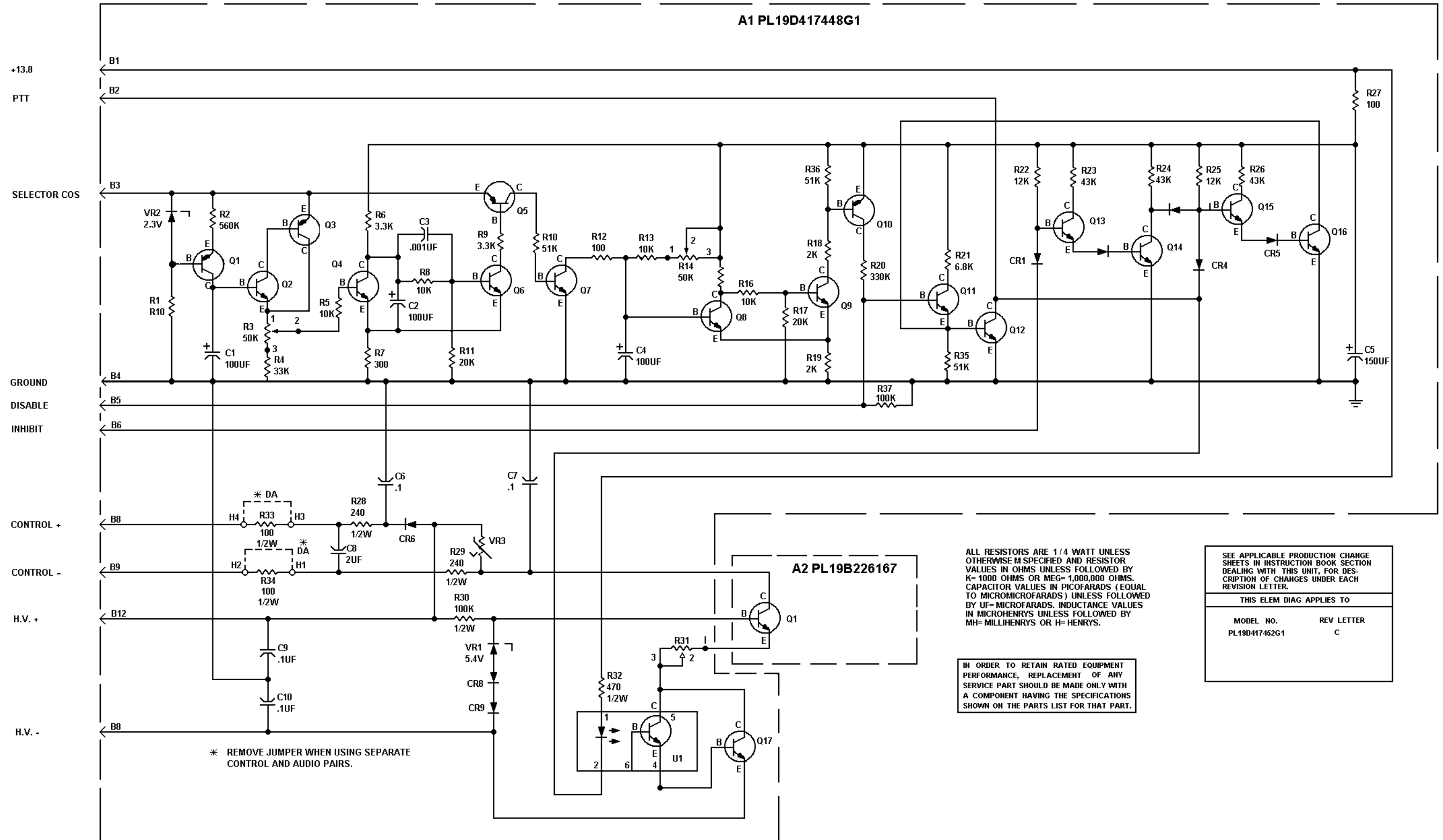
KEYING LOGIC & DC CONTROL BOARD 19D417452G1
