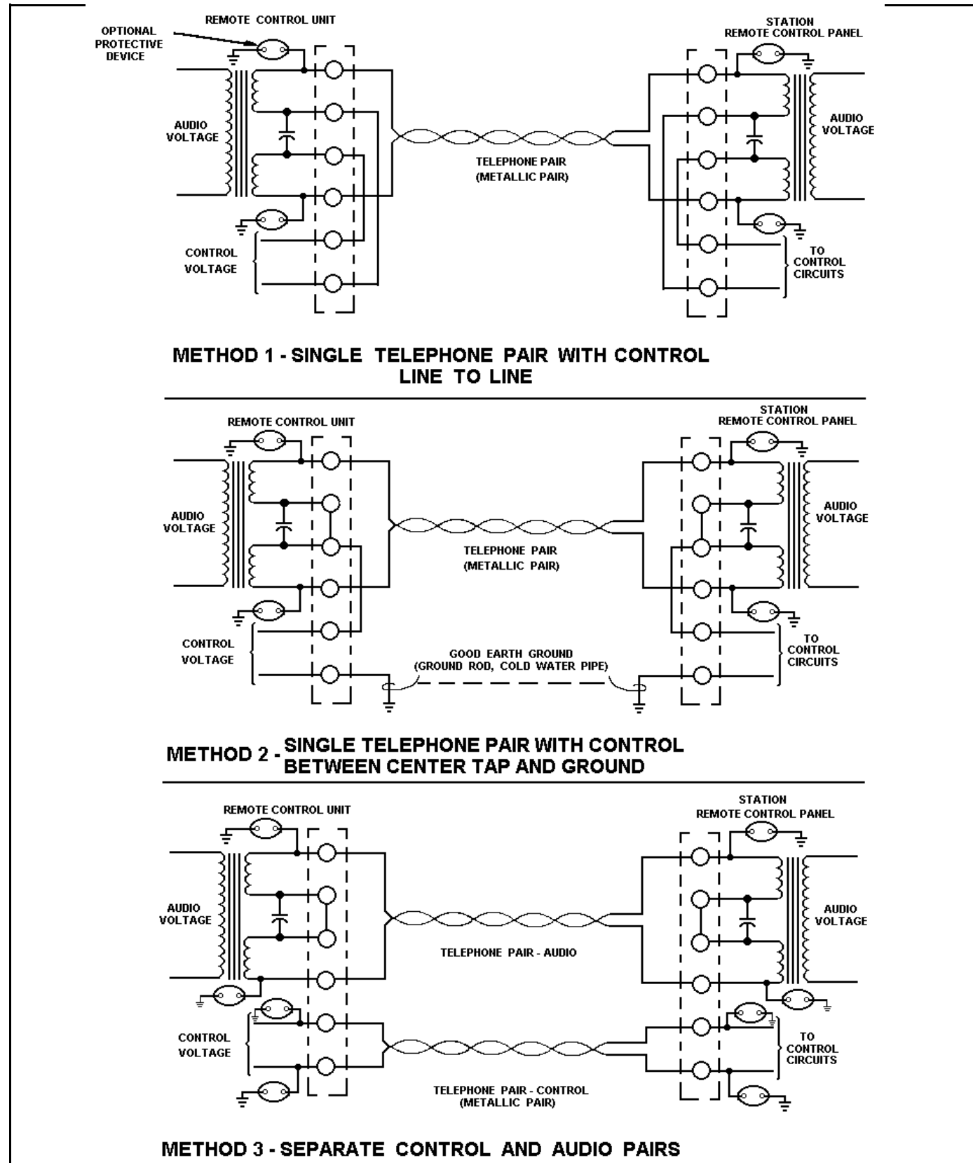
Figure 1 - Telephone Line Connections
