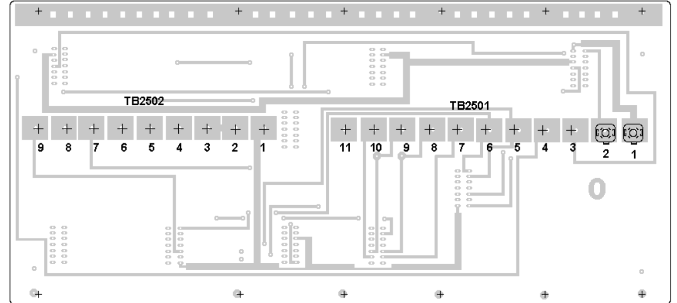
BACK PLANE BOARD 19C320833G2
