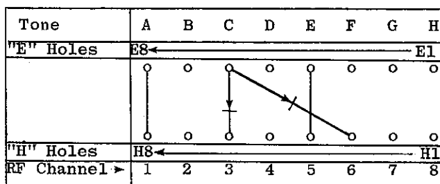
Tone C Duplicating Diode Matrix
