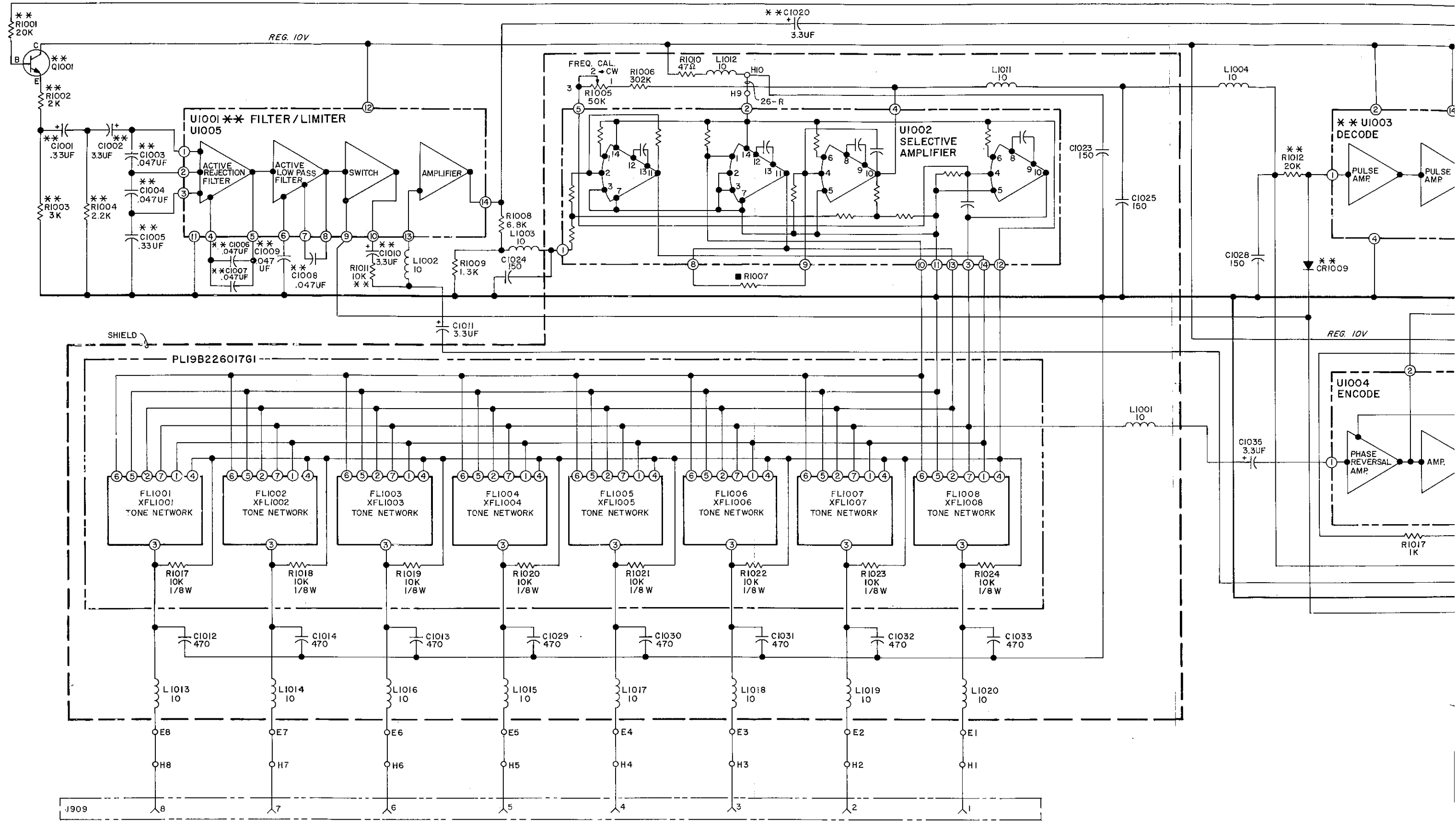
SCHEMATIC DIAGRAM MULTI-TONE ENCODE/DECODE
