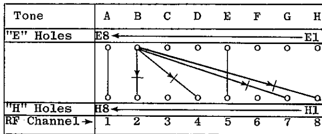
Tone B Duplicating Diode Matrix
