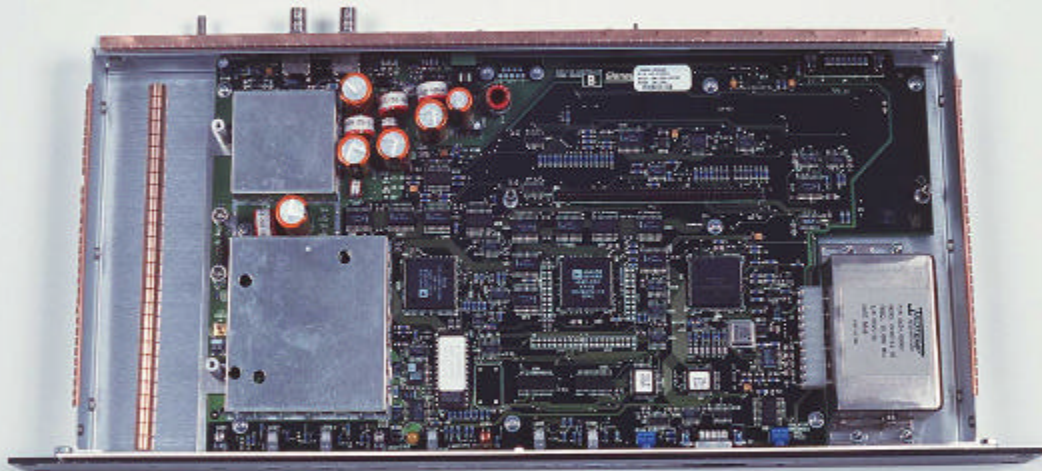
GL-T8200 EXCITER WITH BOARDS OUT
