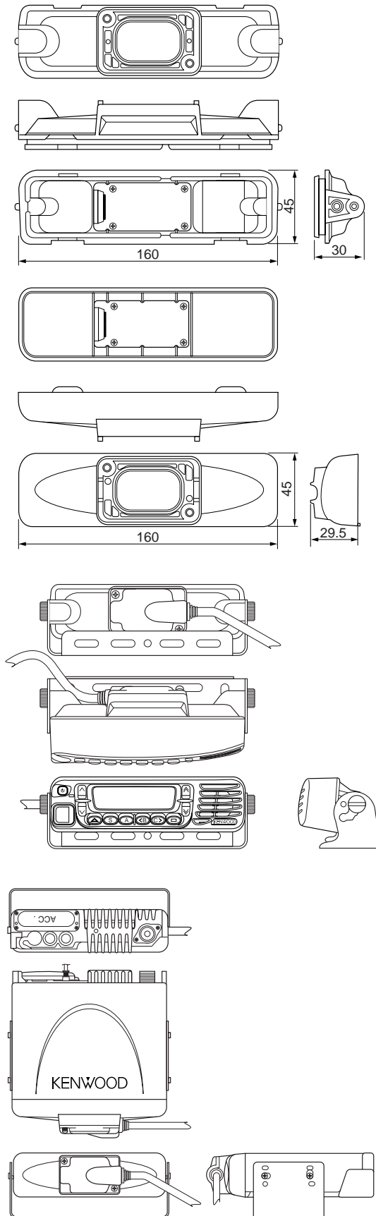
Figure 2-7 Appearance
