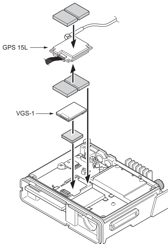
Figure 3-5 Install GPS with VGS-1
