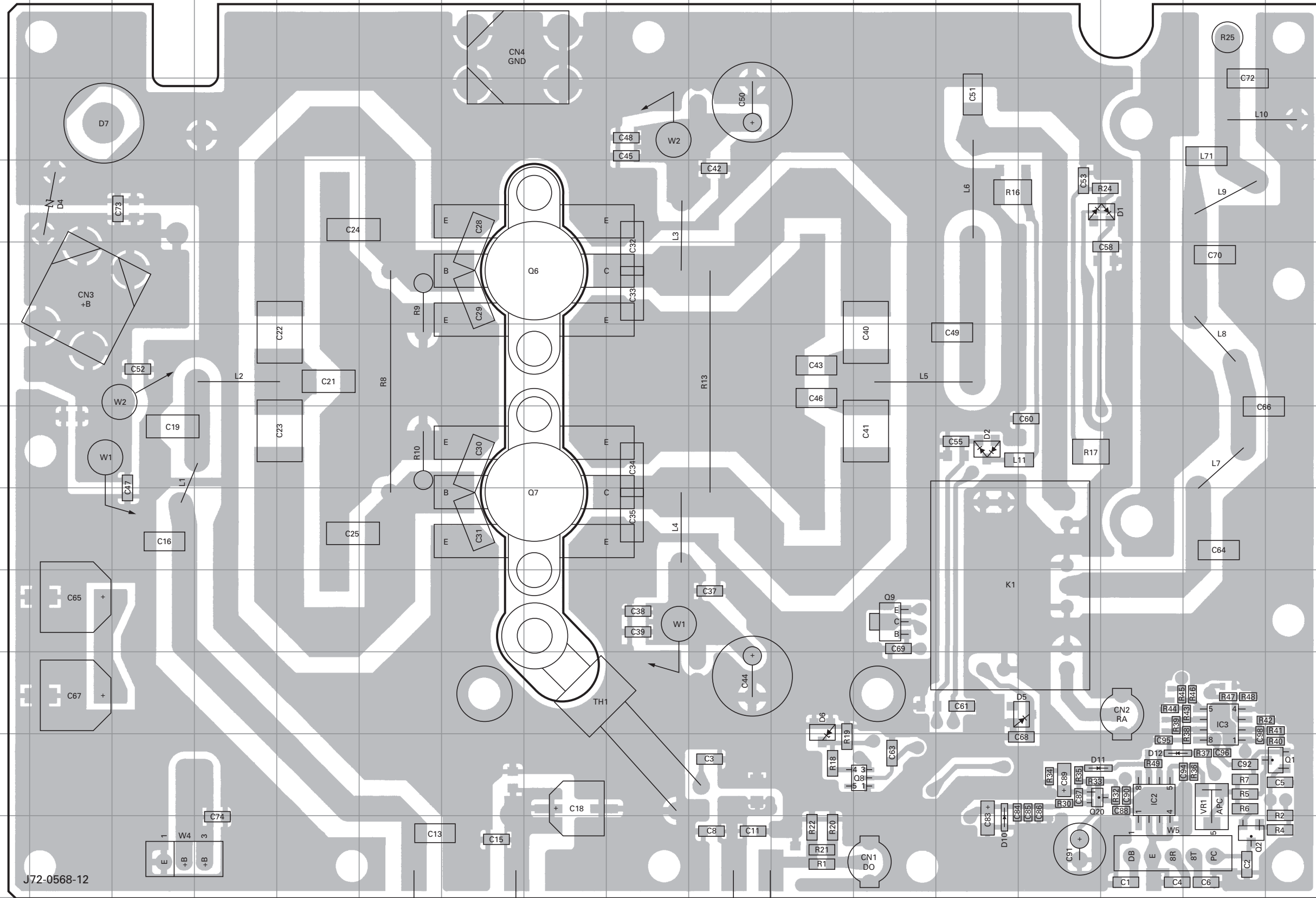
FINAL UNIT (X45-3560-10) Component side view (J72-0568-12)
