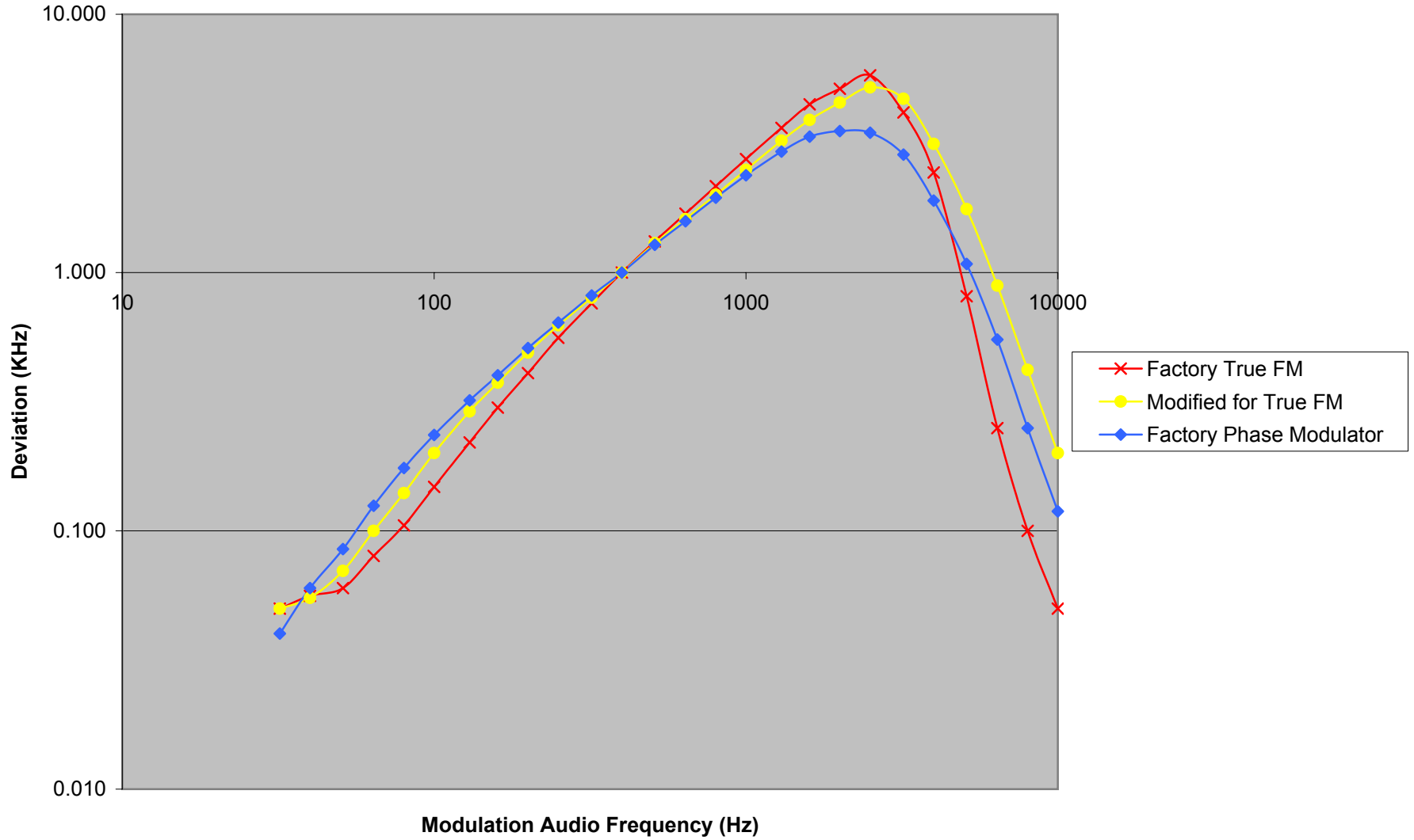
Micor Highband Exciter Frequency Response
