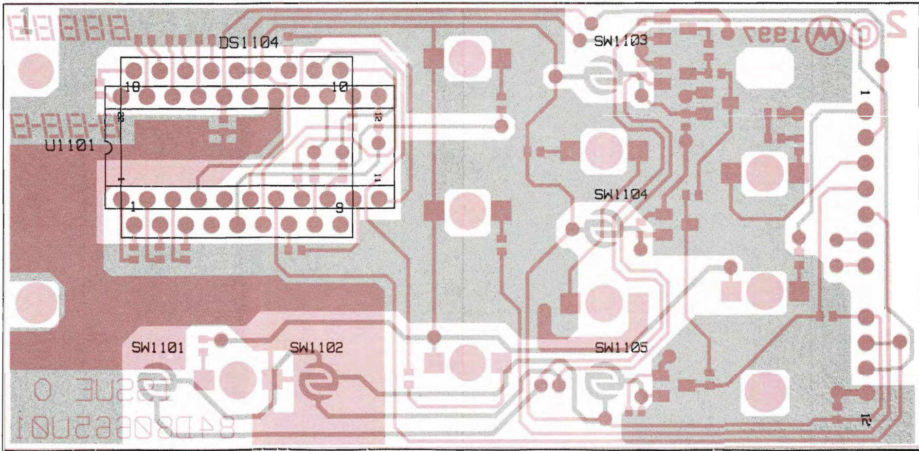
COMPONENT SIDE 84-80665U01 ISSUE 0
