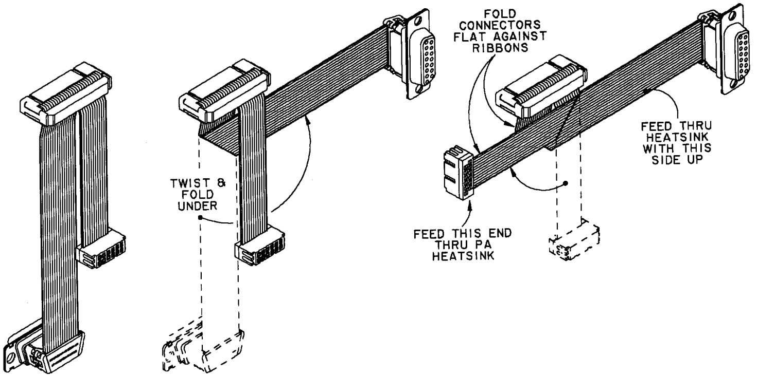
FOLDING RIBBON CABLE FOR INSTALLATION
