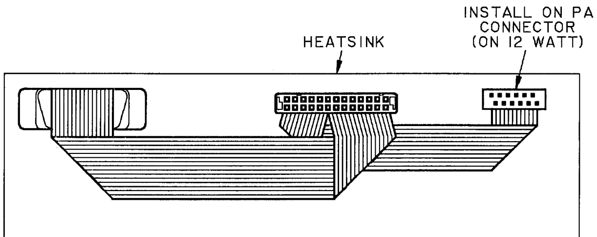
INSTALLING RIBBON CABLE (12-WATT)
