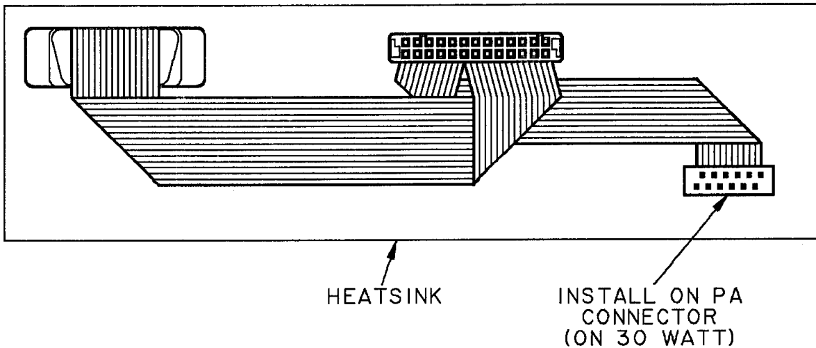
INSTALLING RIBBON CABLE (30-WATT) ALSO 45-WATT AND 50-WATT
