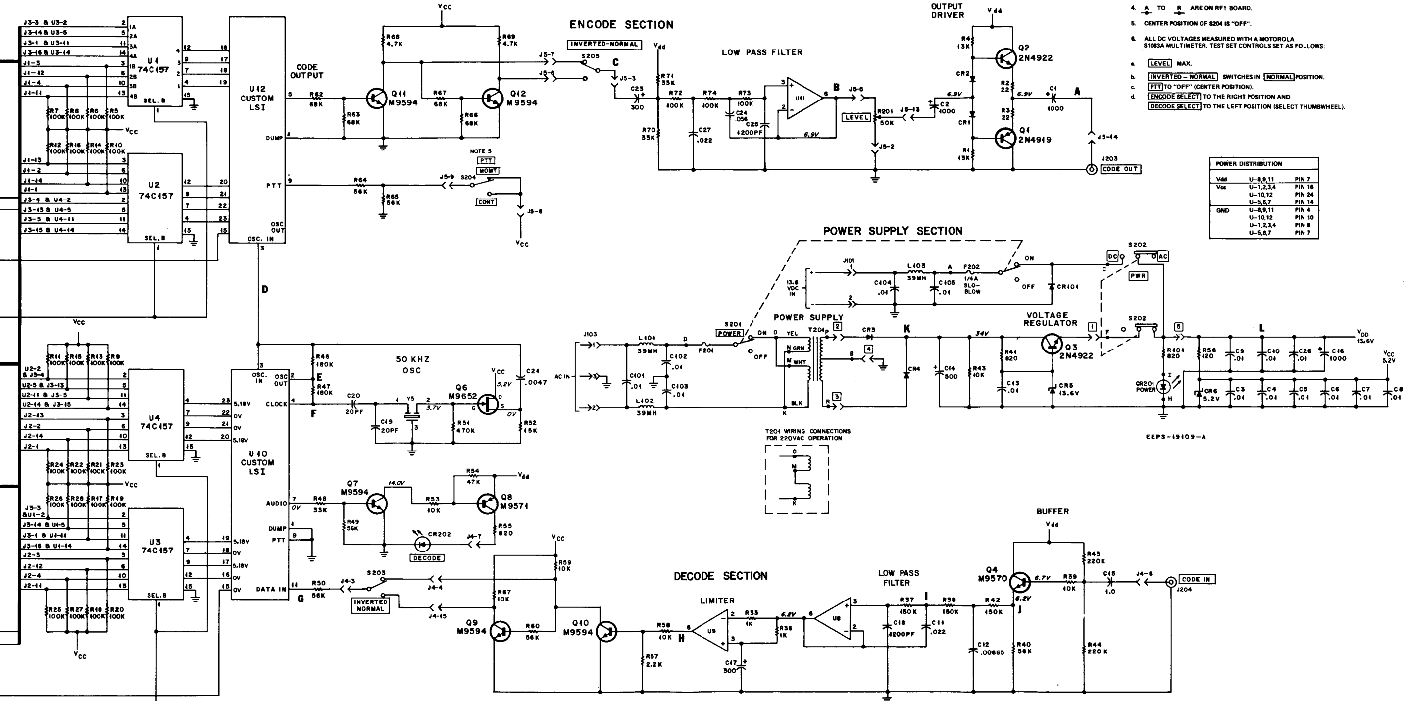
SLN-6413A "Digital Private-Line" Test Set Schematic Diagram and Circuit Board Detail (Motorola No. PEPS-19335-A Sheet 2 of 2) 11/11/75-
