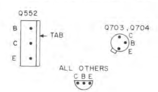
TRANSISTOR BASE DETAILS (SHOWN FROM COMPONENT SIDE)
