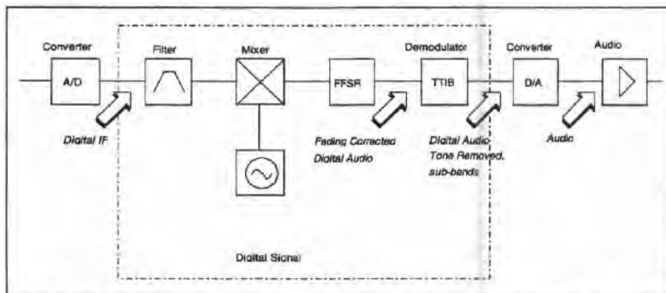
Fig. 8-2 LM Receiver AF
