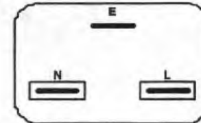
IEC MAINS PLUG (PL1) (view onto rear pins)
