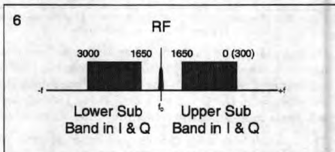
Figure 3-5 Up-convert to RF to Give Transmitted Signal
