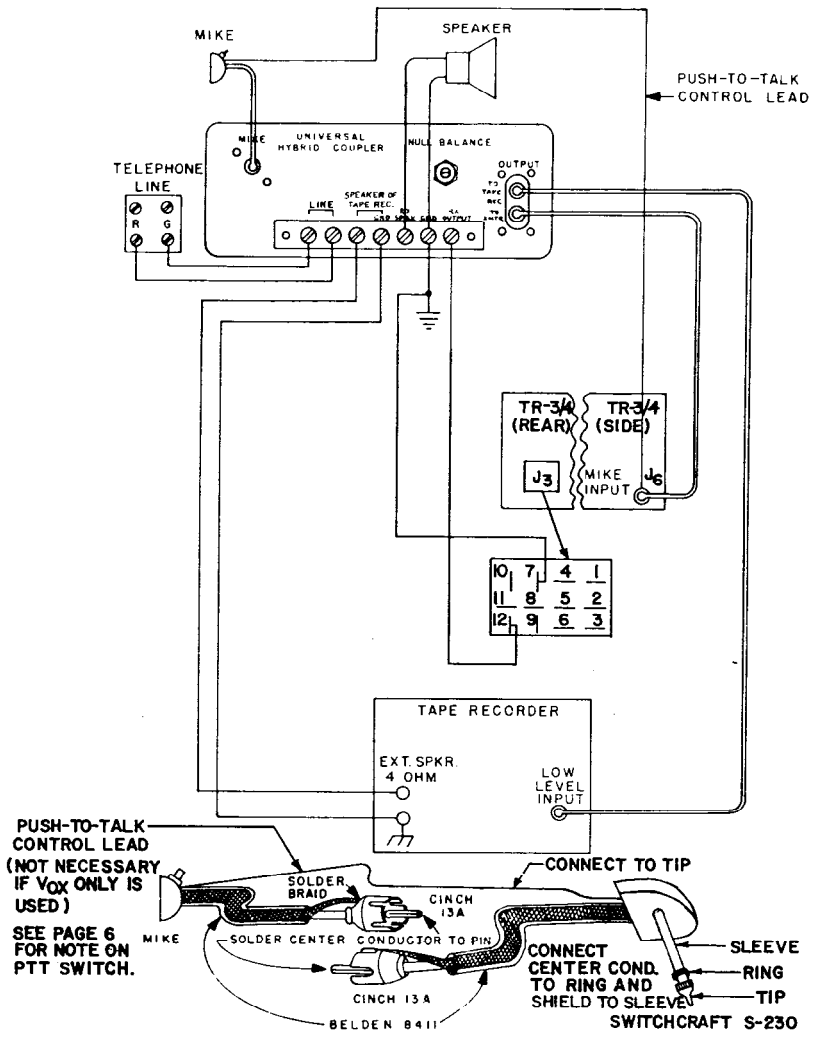
FIG. 11 TYPICAL INSTALLATION FOR DRAKE TR-3/TR-4 M-B348-32 A/10-63
