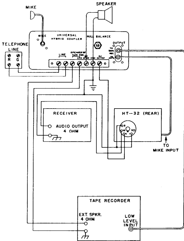
FIG. 6 TYPICAL INSTALLATION WITH HALLICRAFTERS HT-32 TRANSMITTER M-8348-25AW/10-63
