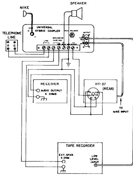
FIG. 7 TYPICAL INSTALLATION M-8348-26AA/5-66 WITH HALLCRAFTERS HT-37 TRANSMITTER
