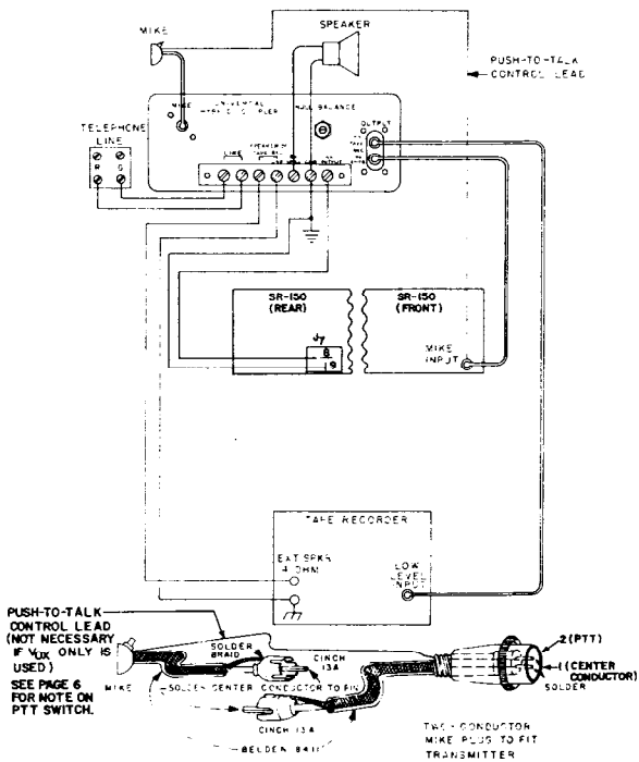
FIG. 8 TYPICAL INSTALLATION WITH M-8349-27AA/10-63 HALLCRAFTERS SR-150
