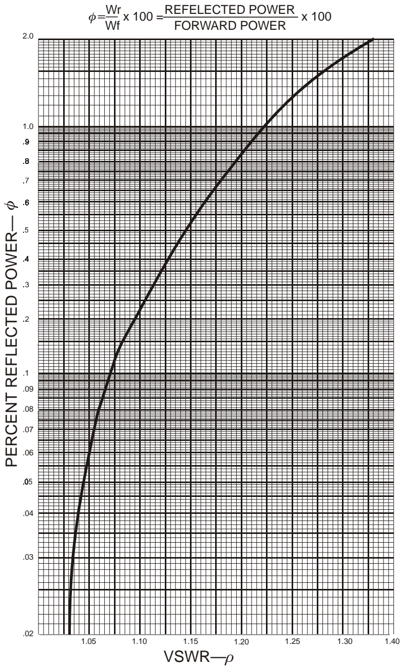
Figure 4 Percent Reflected Power vs. VSWR (1.0 – 8.0)
