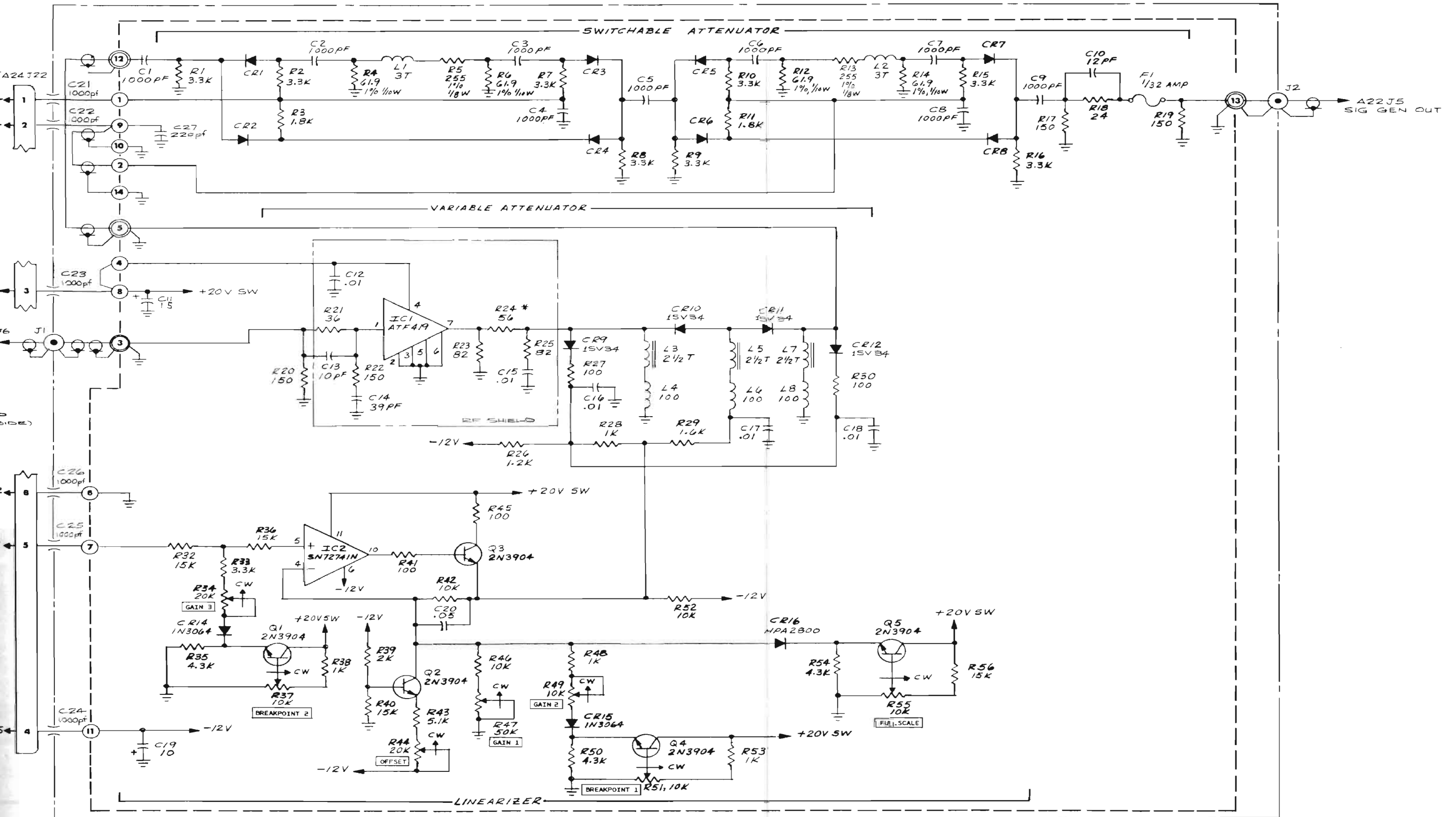
Figure 6-25. Output Attenuator. A20
