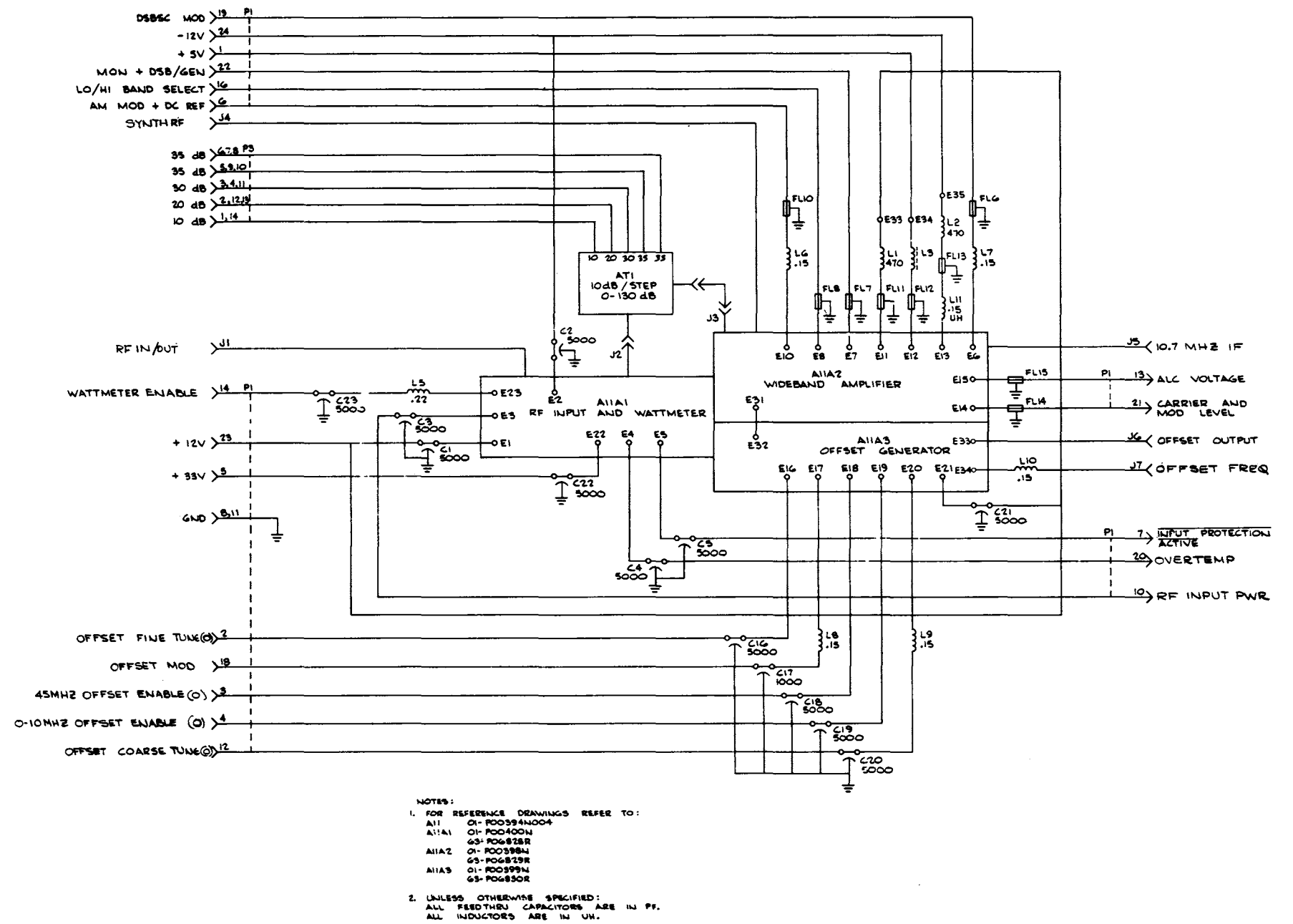
Figure 17-3. RF Input Module A11 with IEEE Option Schematic Diagram
