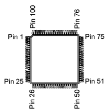
HD64F2238BFA (Q3014)
