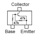
DTC144EE (26) (Q3046, 3052, 3053)
