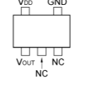
BD4845FVE (Q3012)
