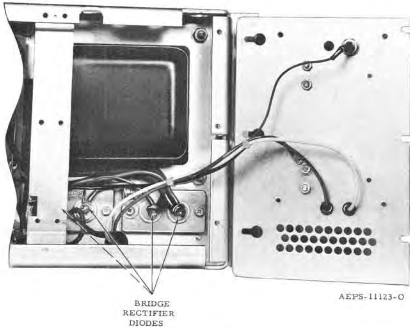
Figure 7. Access to Bridge Rectifier Circuit
