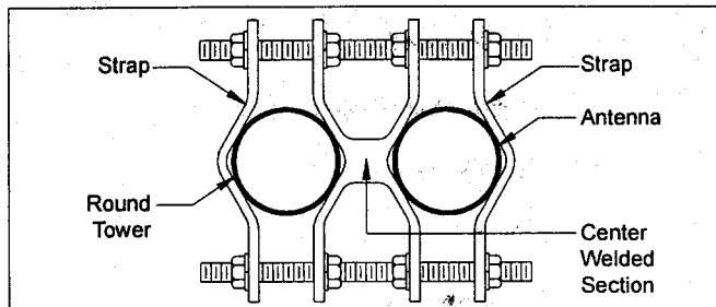
Figure 1. Mounting on Round Tower Legs.
