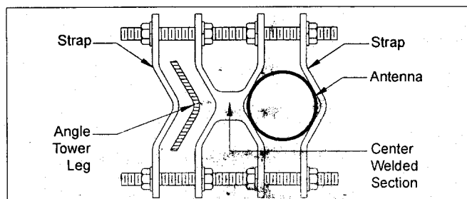
Figure 2. Mounting on Angle Tower Legs.
